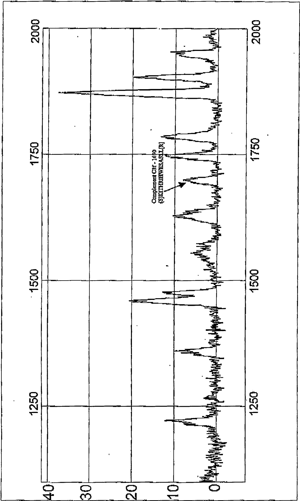
SPECTRA SHOWING DISEASE INDICATIVE MARKER FIGURE 2
