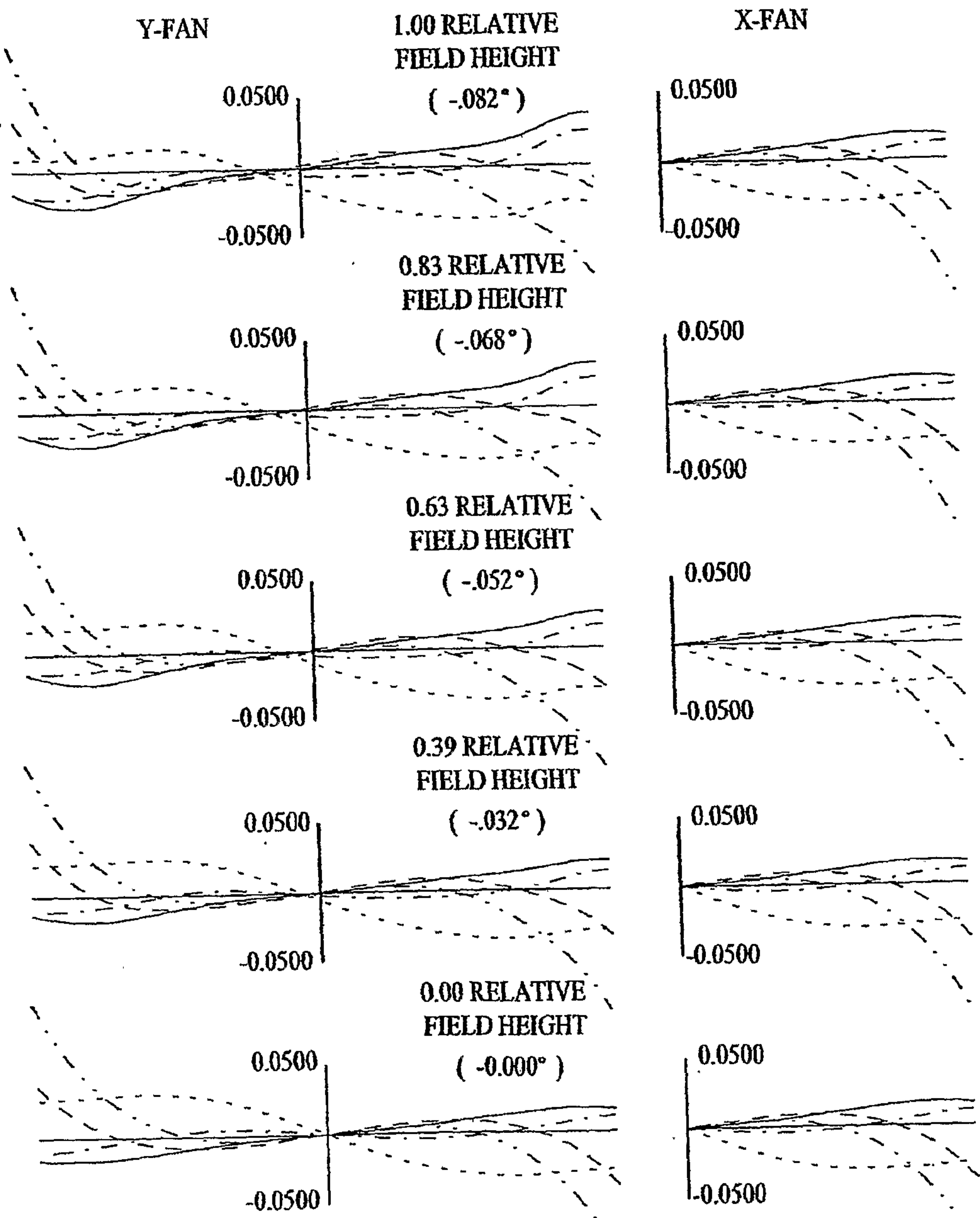
Fig. 53 RAY ABERRATIONS (MILLIMETERS) POSITION 15 ----- 643.8469 NM ----- 587.5600 NM ----- 546.0700 NM ----- 486.1300 NM ----- 460.0000 NM
