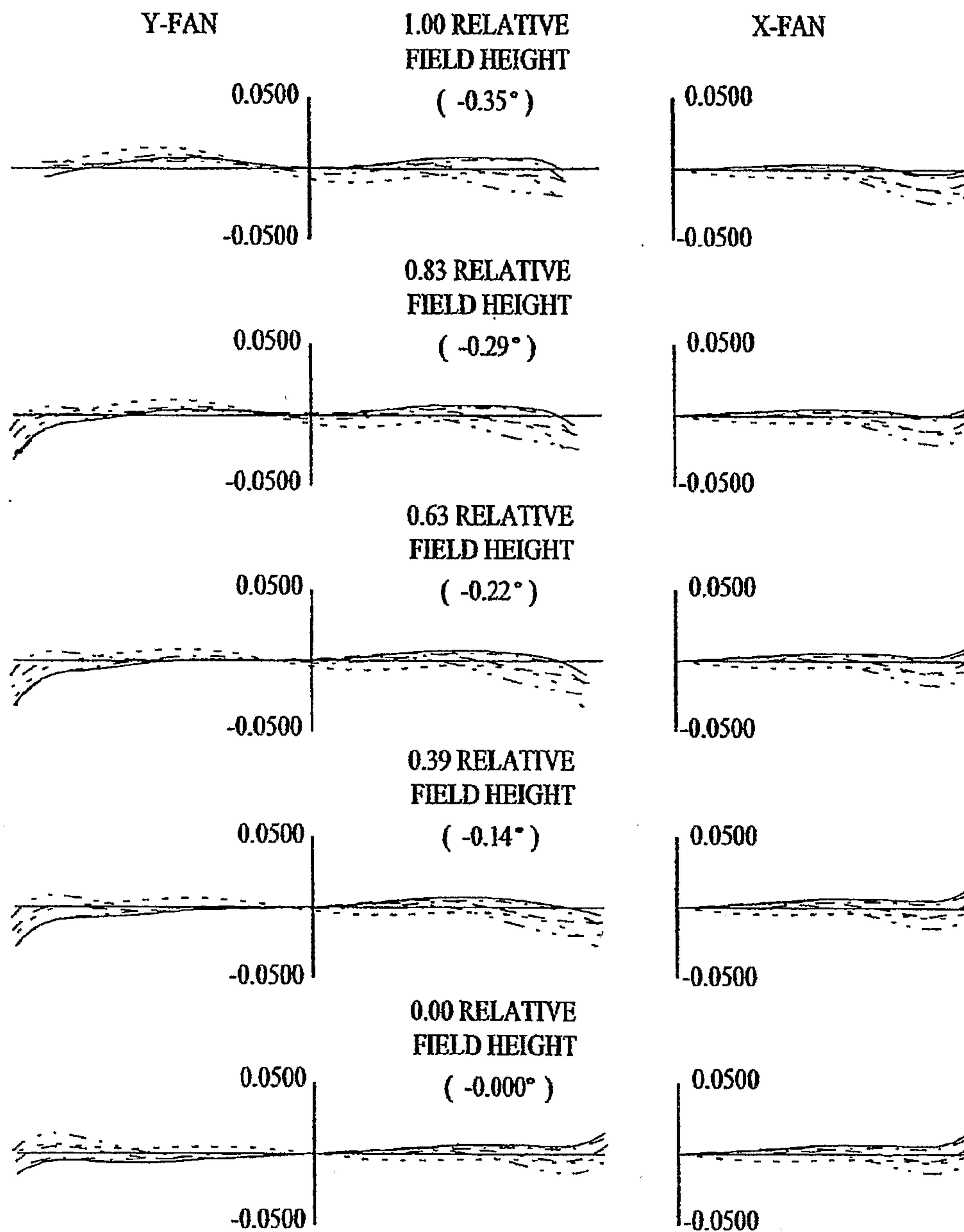
Fig. 54 RAY ABERRATIONS ( MILLIMETERS ) POSITION 16
