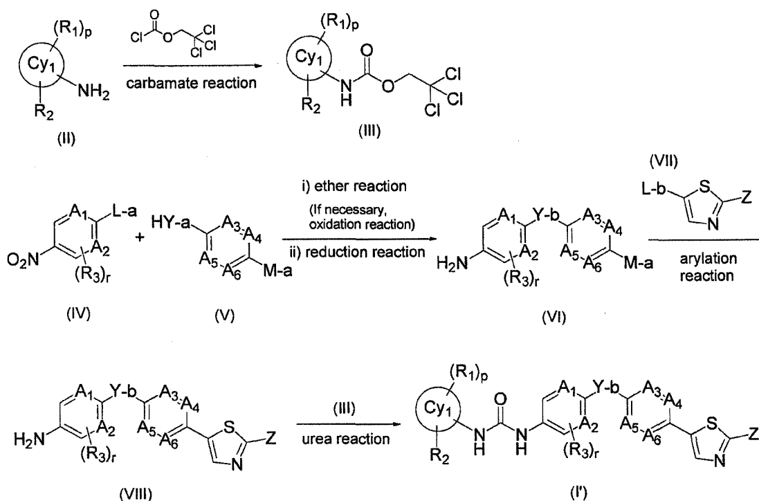
Reaction Scheme 1
