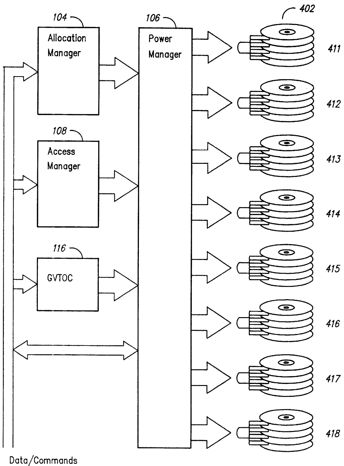
EXEMPLARY PHYSICAL LAYOUT FOR LOW POWER APPLICATIONS
