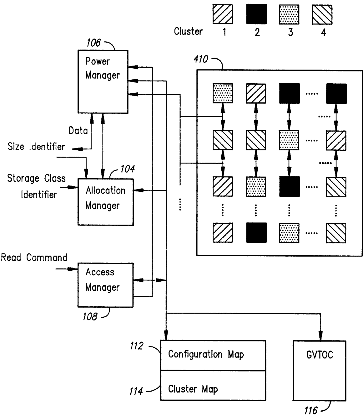
DATA FLOW FIG. 3
