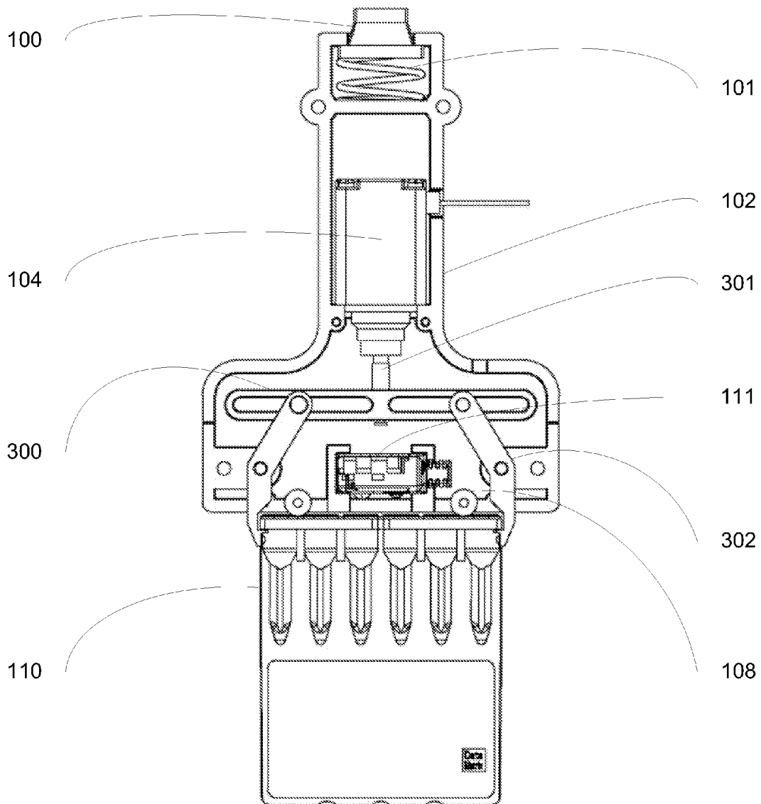
Fig. 4 -- Configuration 2 Closed with Cassette
