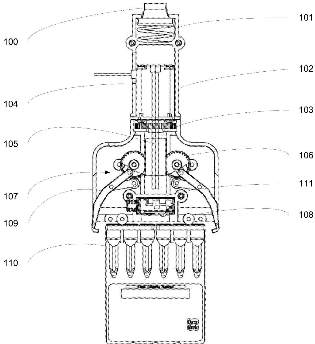
Fig. 1 -- Configuration 1 Open with Cassette
