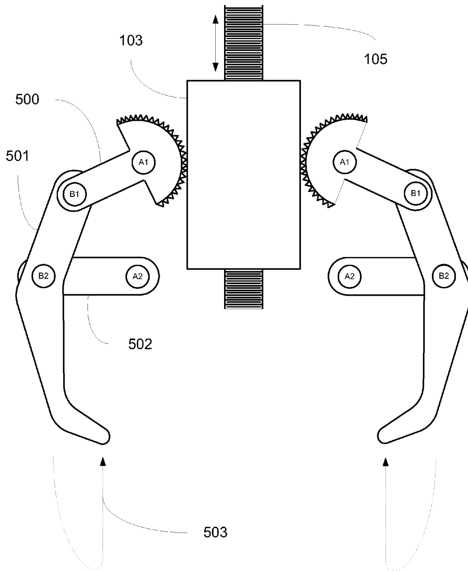
Fig. 5 -- Configuration 1 Linkage Details (Not to Scale)
