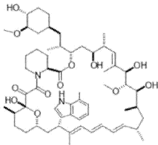
Scheme 1. Structure of AP21967
