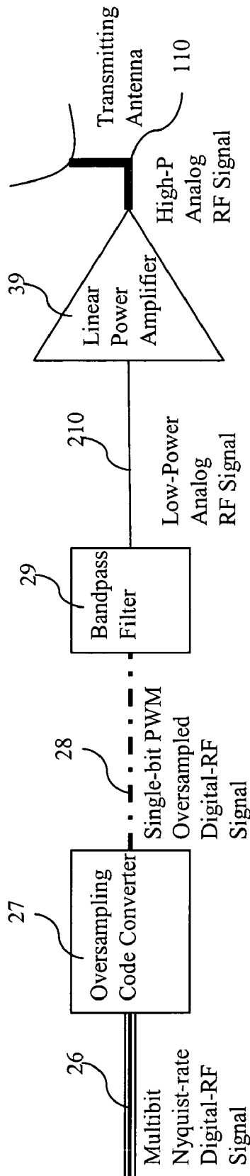
Fig. 3A Prior Art
