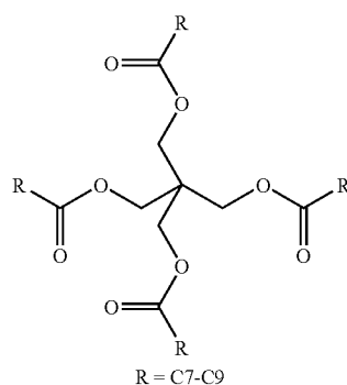
pentaerythrityl tetracaprylate
