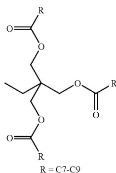
trimethylpropane tricaprylate
