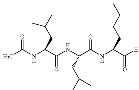
N-Acetyl-Leu-Leu-Nle-CHO
