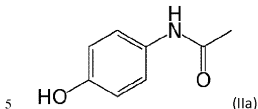
Paracetamol
