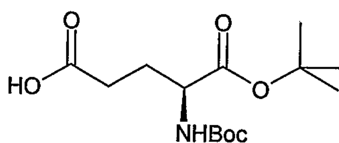
(S)-2-tert-Butoxycarbonylamino-pentanedioic acid 1-tert-butyl ester
