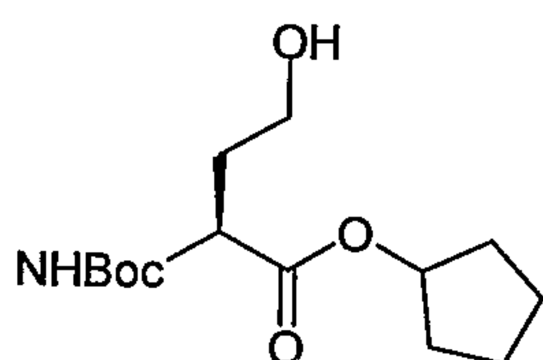
(S)-2-tert-Butoxycarbonylamino-4-hydroxy-butyric acid cyclopentyl ester
