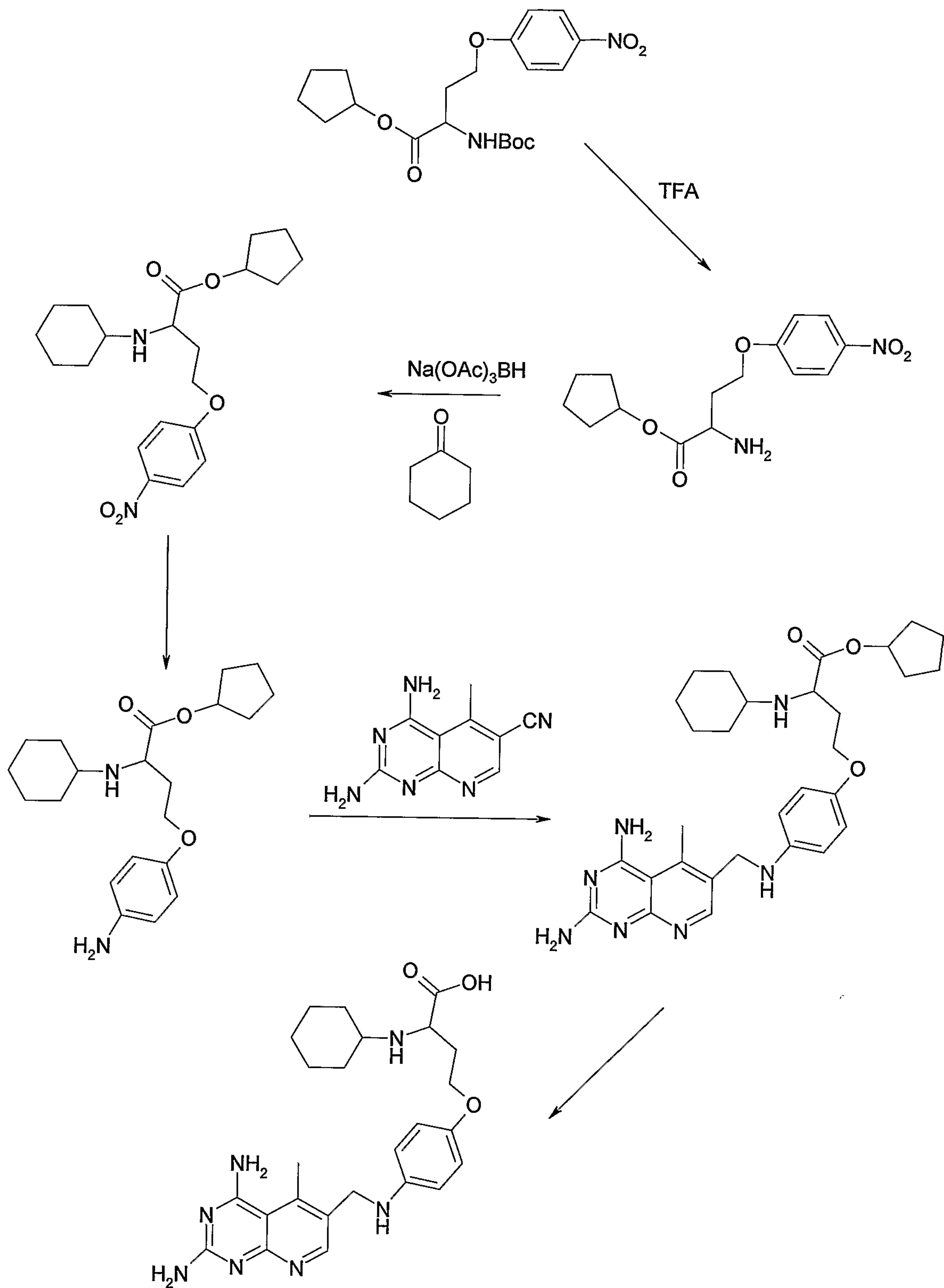
Scheme IV
