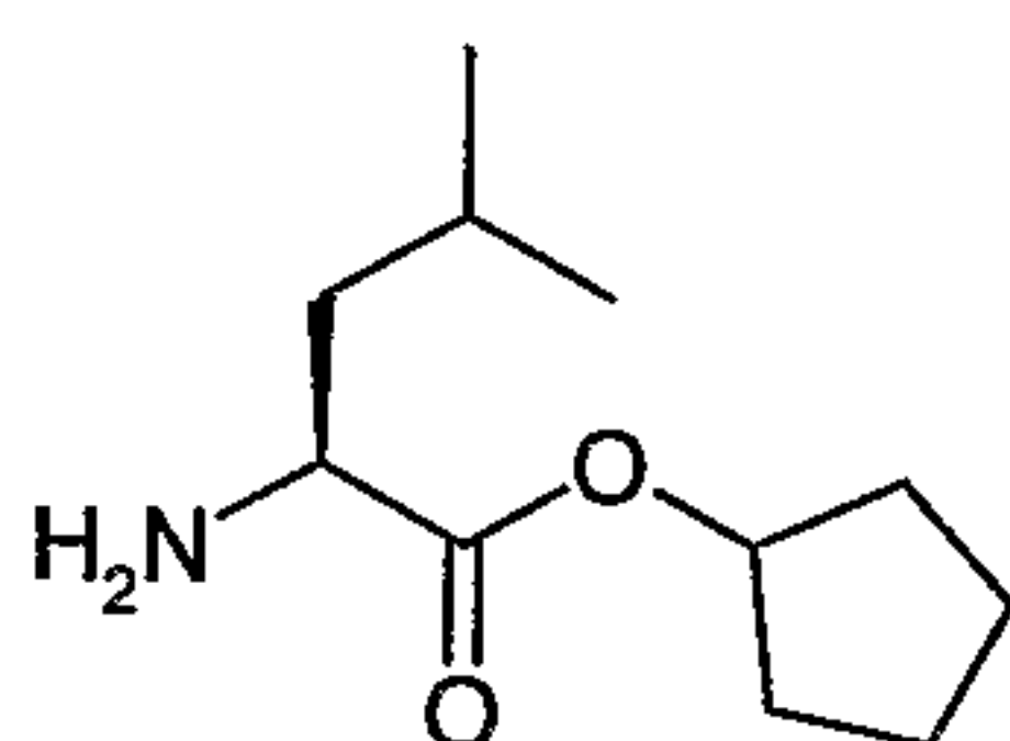
(S)-2-Amino-4-methyl-pentanoic acid cyclopentyl ester
