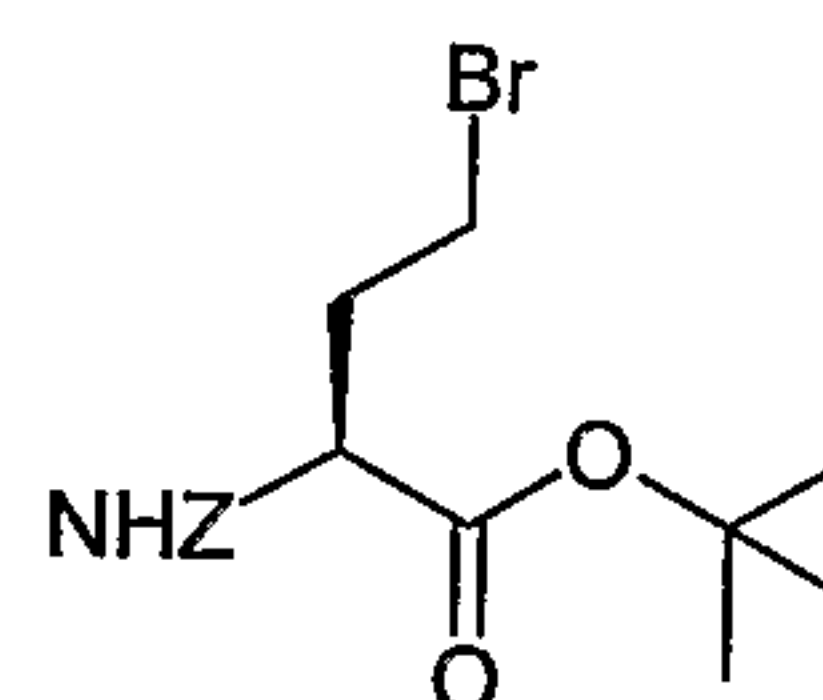
(S)-2-Benzyloxycarbonylamino-4-bromo-butyric acid tert-butyl ester
