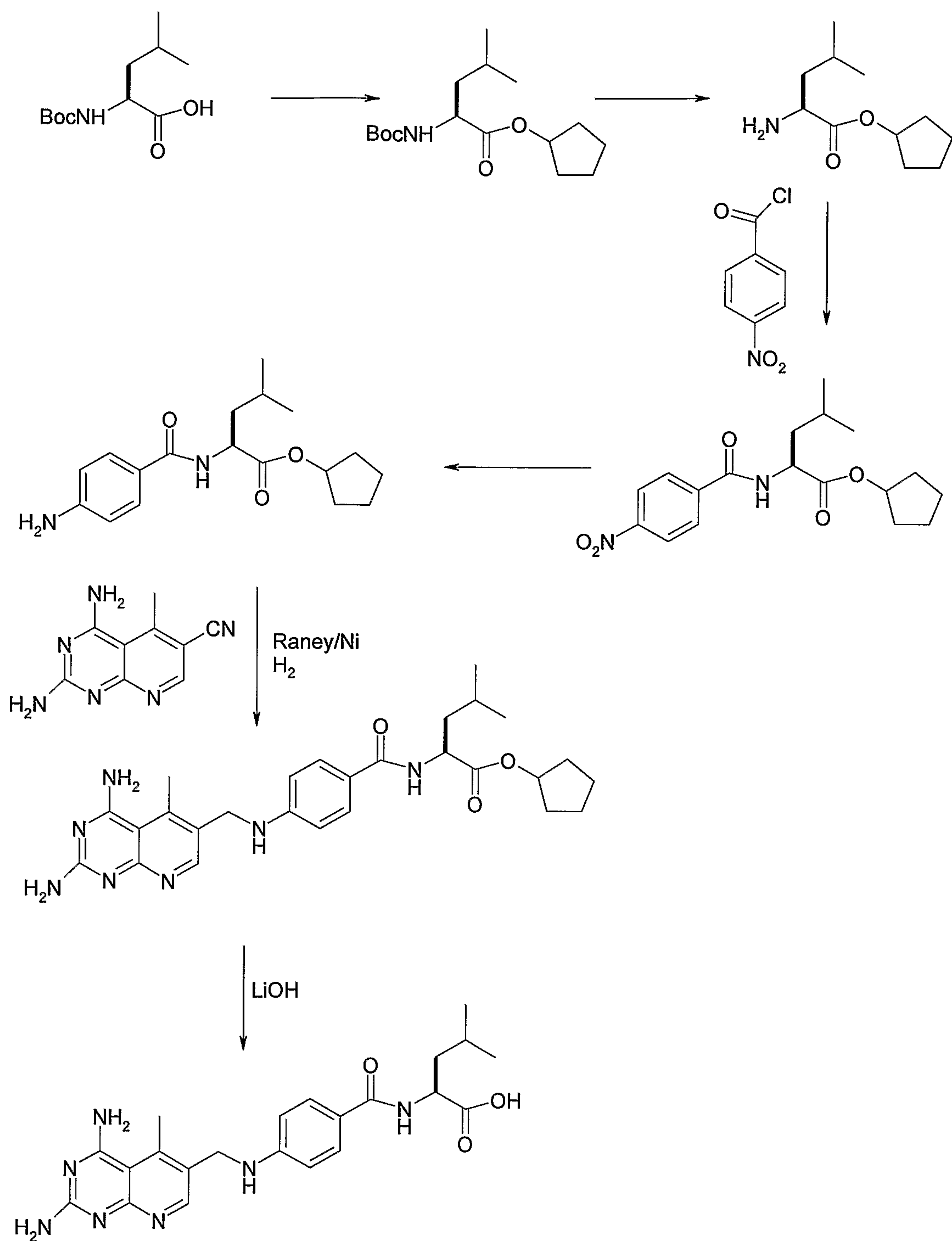
Scheme I
