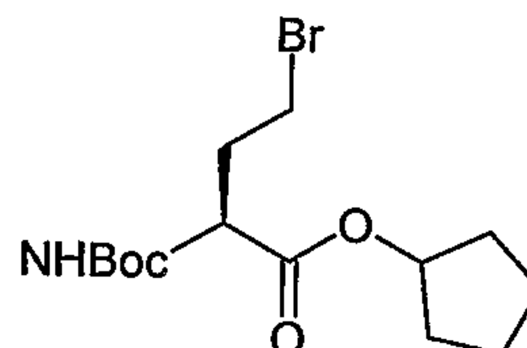
(S)-4-Bromo-2-tert-butoxycarbonylamino-butyric acid cyclopentyl ester
