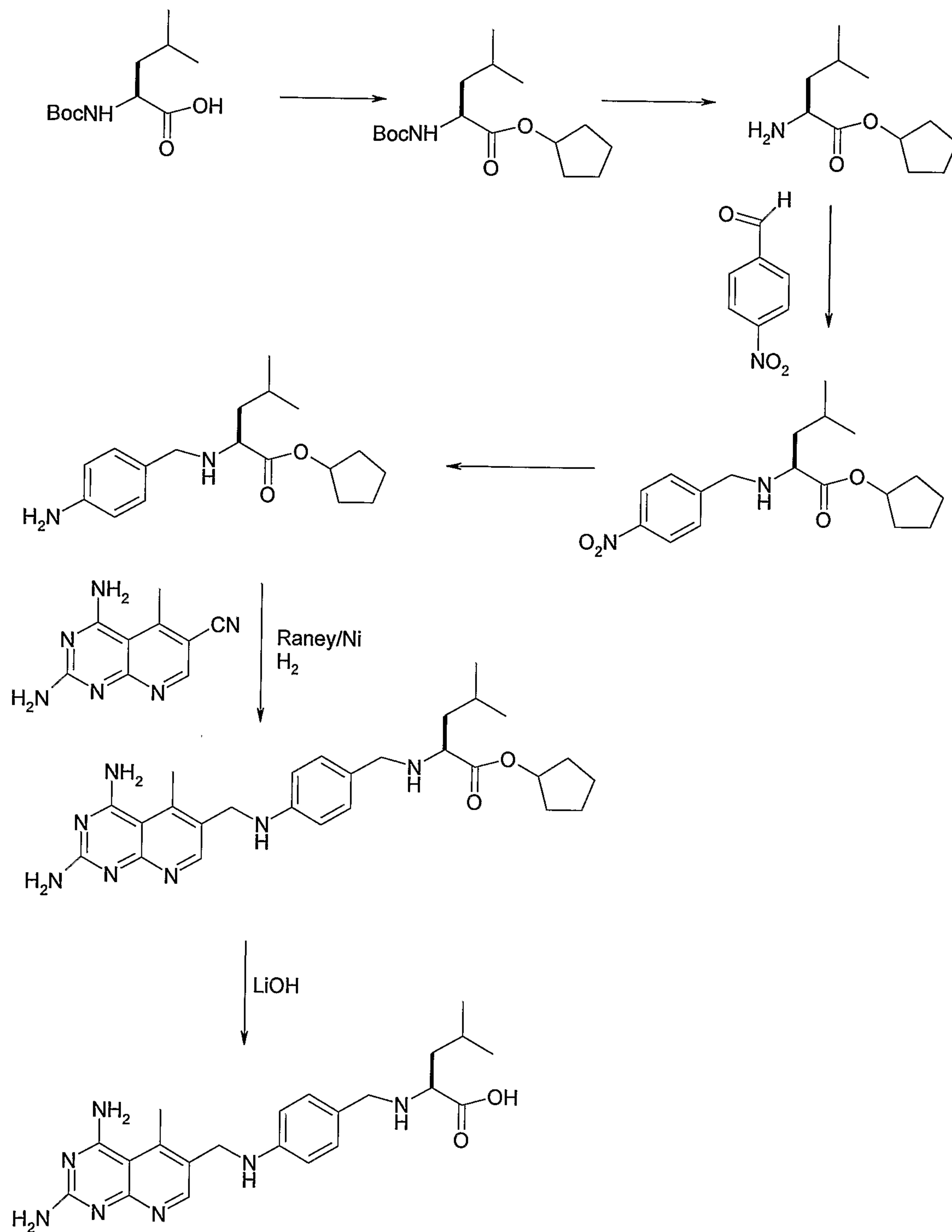
Scheme II
