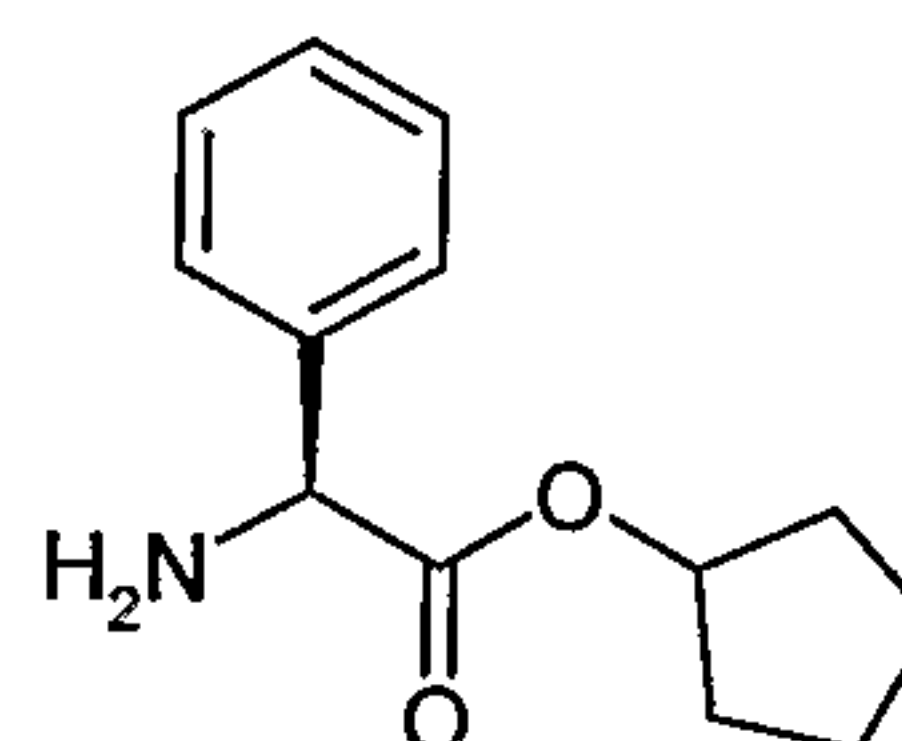
(S)-Amino-phenyl-acetic acid cyclopentyl ester
