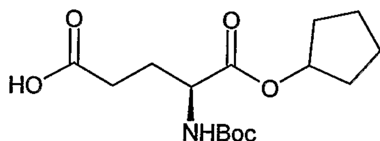
(S)-2-tert-Butoxycarbonylamino-pentanedioic acid 1-cyclopentyl ester
