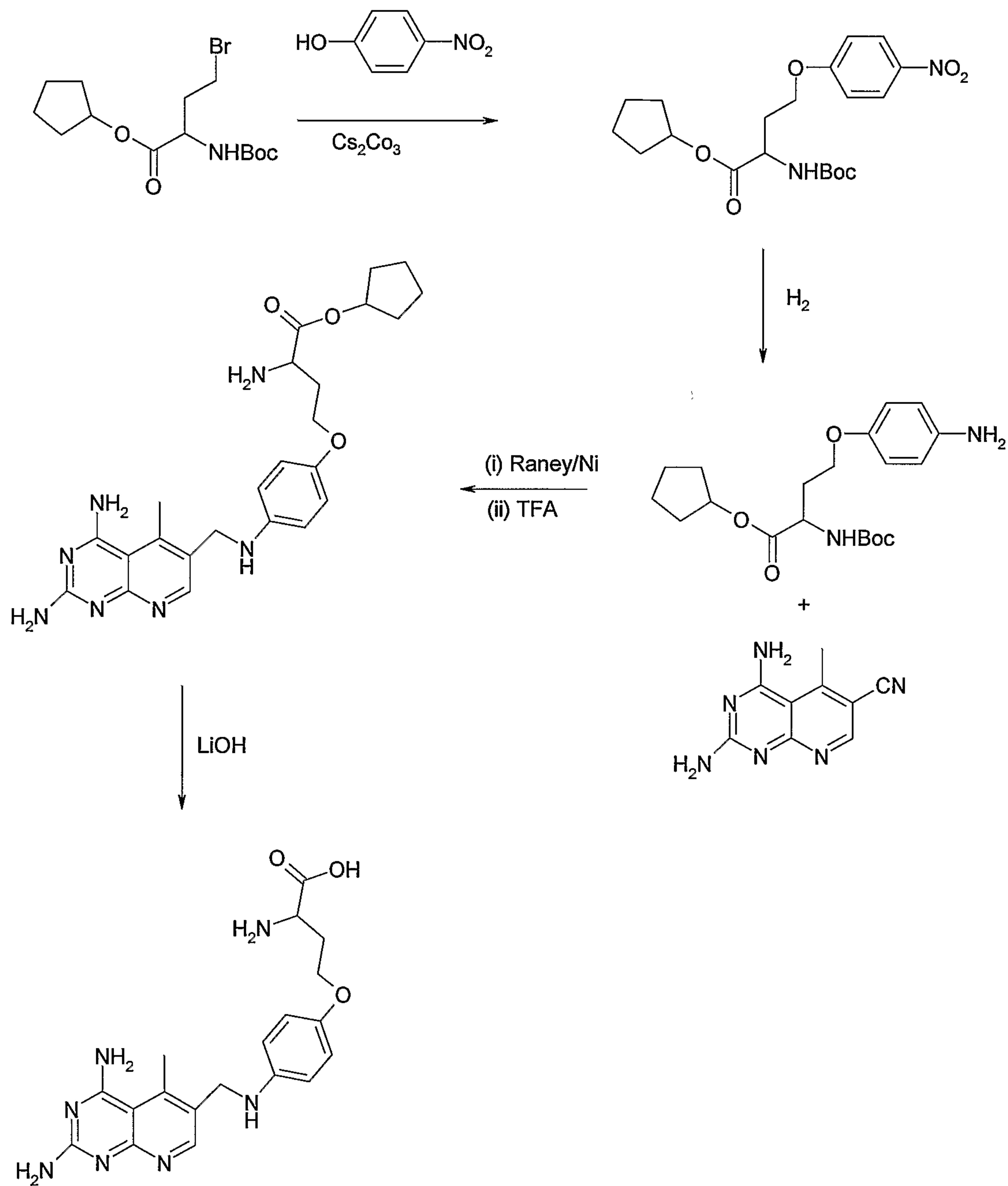
Scheme III
