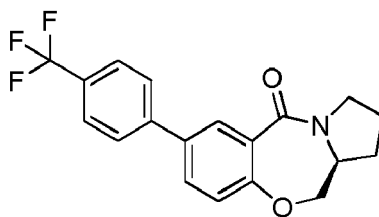
8-(4-(trifluoromethyl)phenyl)-3,4,12,12a-tetrahydrobenzo[f][1,4]oxazino[3,4-c][1,4]oxazepin-6(1H)-one (Compound 11-63) MS m/z : 364 ( MH^+ )
