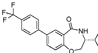
(R)-3-isopropyl-4-(pyrimidin-2-ylmethyl)-7-(4-(trifluoromethyl)phenyl)-3,4-dihydrobenzo[f][1,4]oxazepin-5(2H)-one (Compound 11-78) MS m/z : 442 ( MH^+ )
