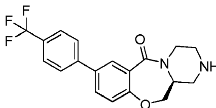
(S)-tert-butyl 6-oxo-8-(4-(trifluoromethyl)phenyl)-3,4,12,12a-tetrahydro-1H-benzo[f]pyrazino[2,1-c][1,4]oxazepine-2(6H)-carboxylate (Compound 11-29) MS m/z : 463 ( MH^+ )
