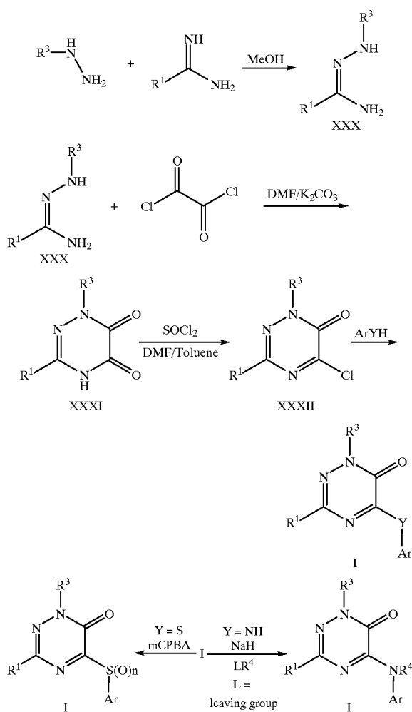
Scheme 6
