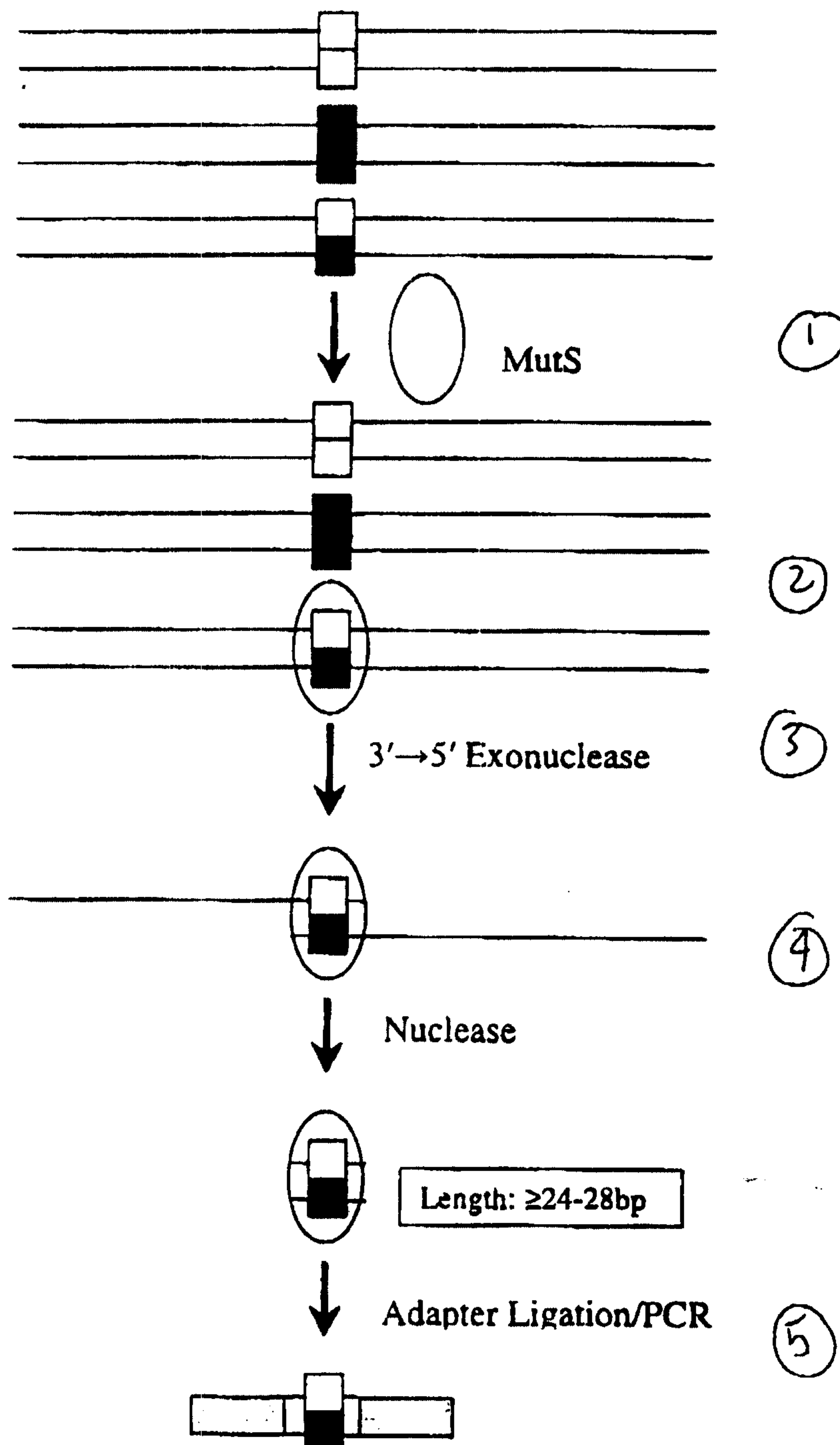
Scheme 1
