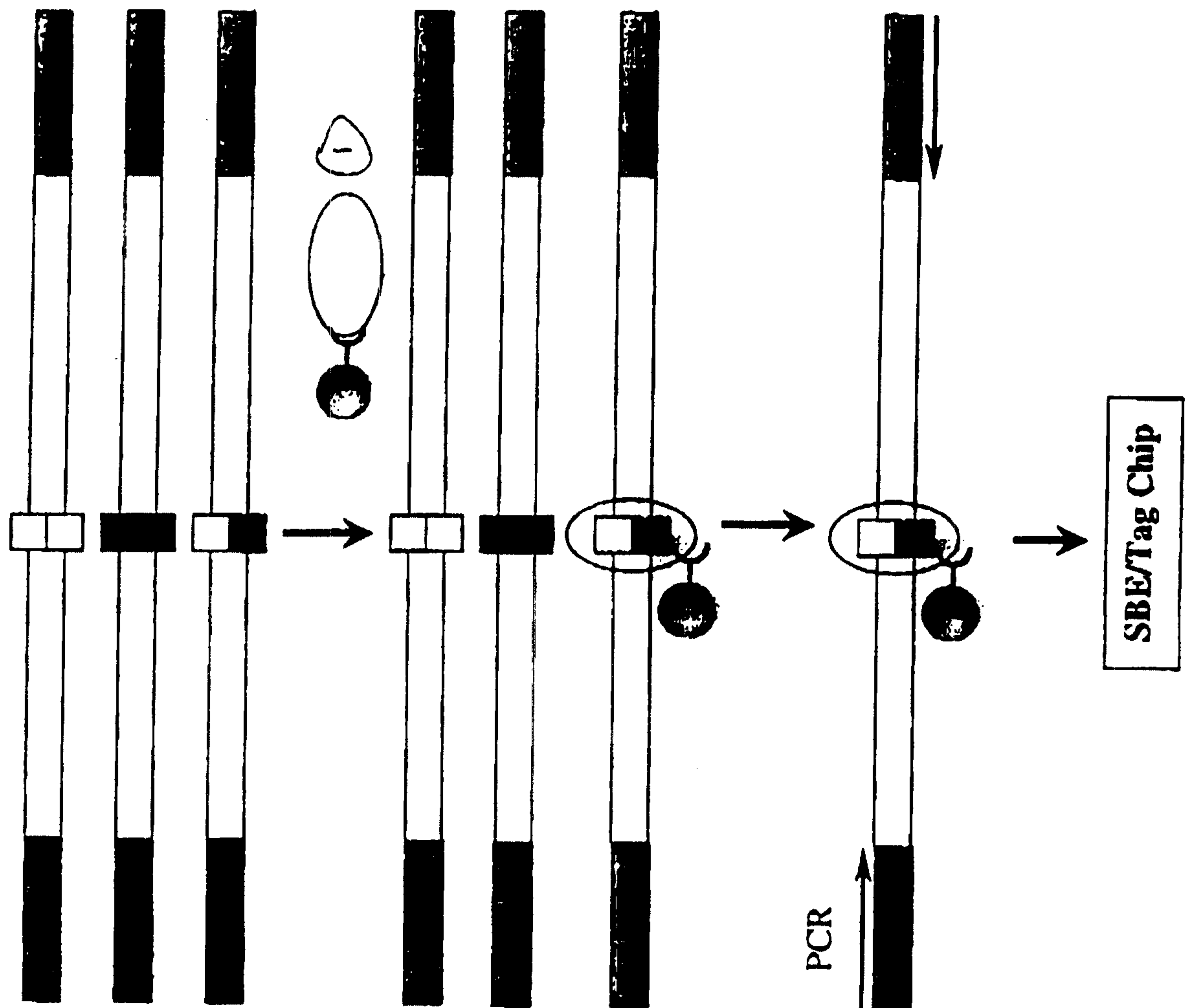
Scheme II
