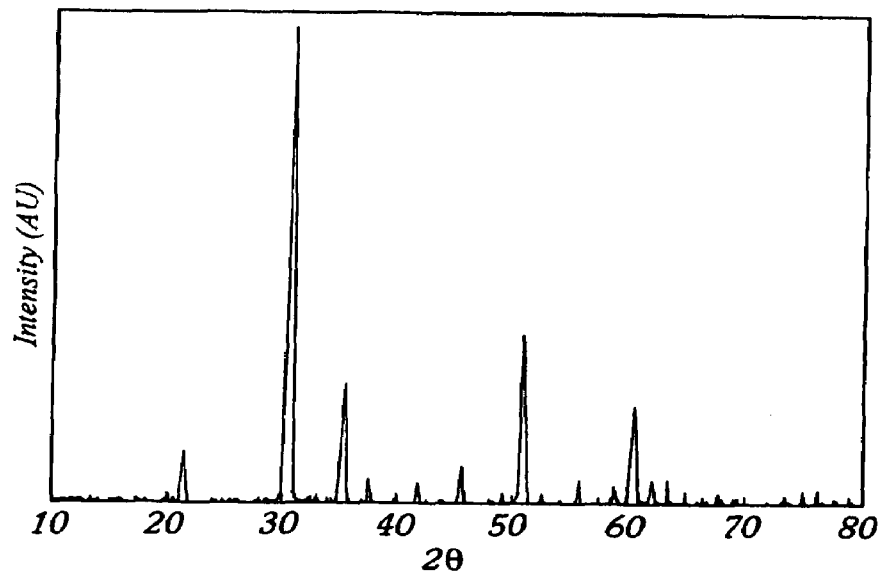
XRD spectra of the indium tin oxide nanopowder
