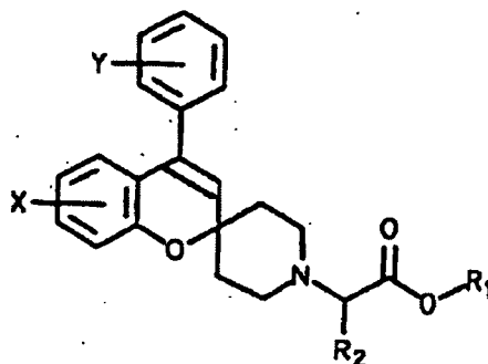
Formel I
