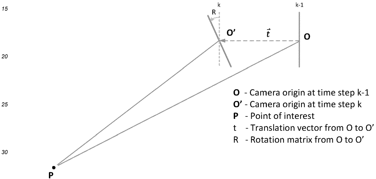
2-D Camera Rotation/Translation Diagram
