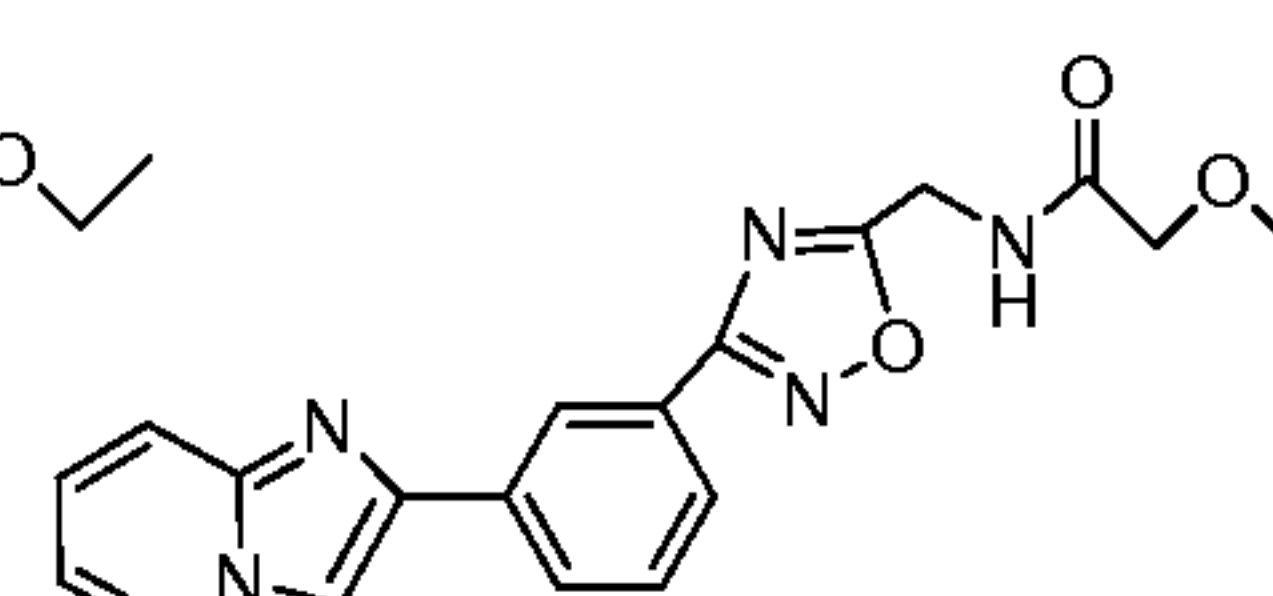
Compound 87
