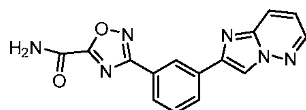
Compound 24
