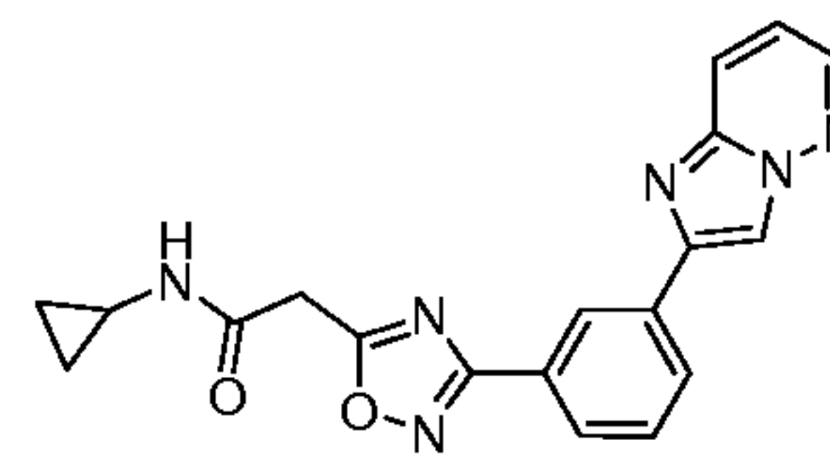
Compound 56
