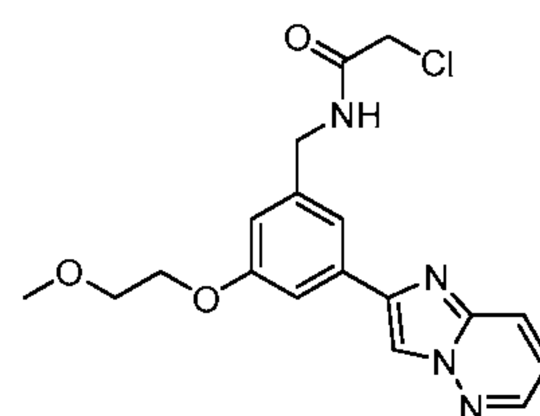
Compound 41
