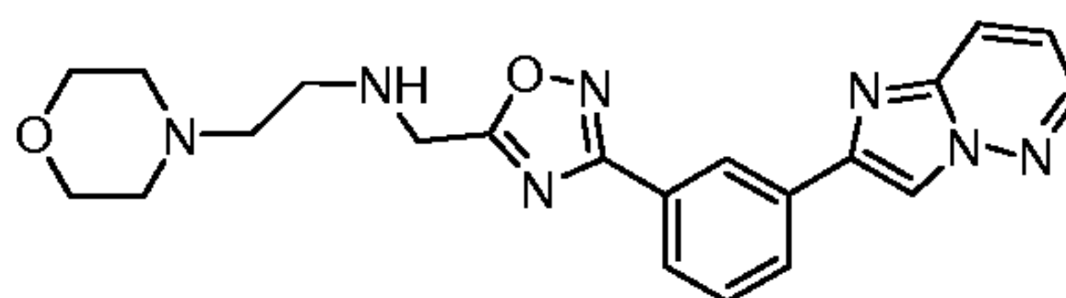
Compound 5
