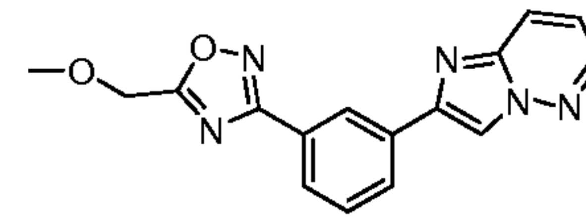
Compound 12
