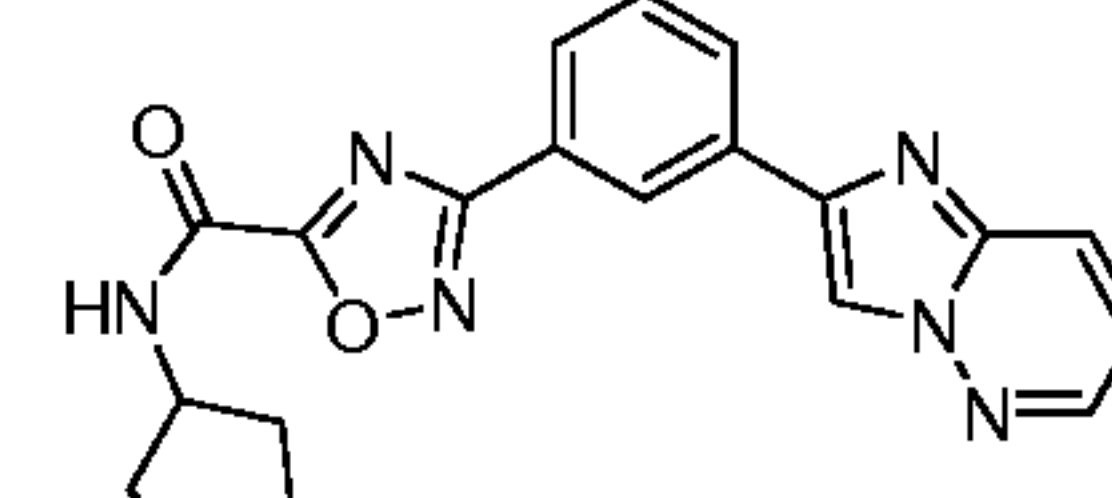
Compound 59
