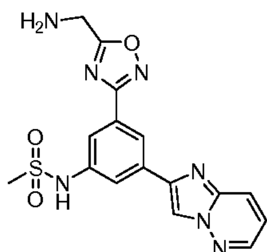
Compound 80
