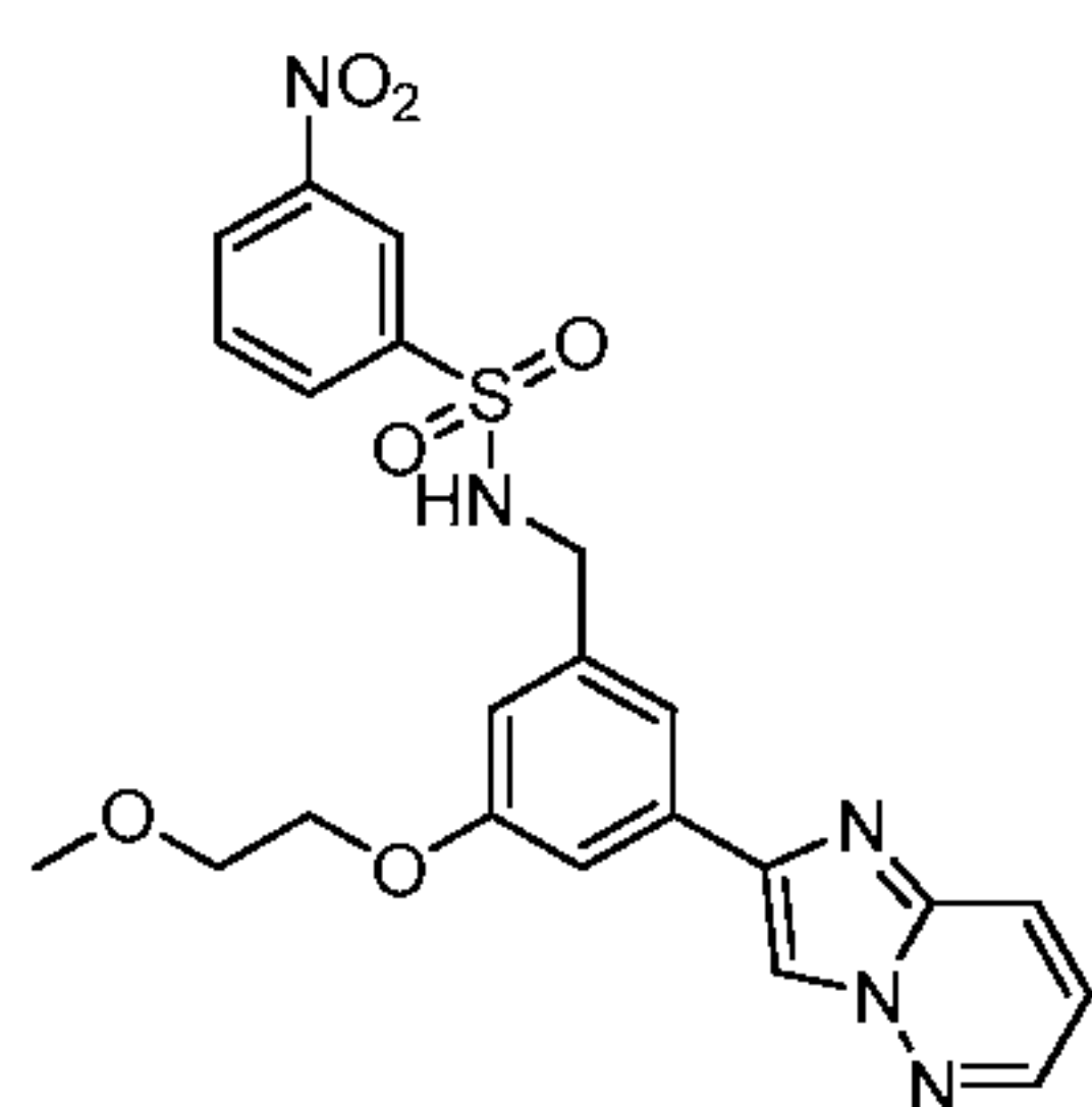
Compound 43
