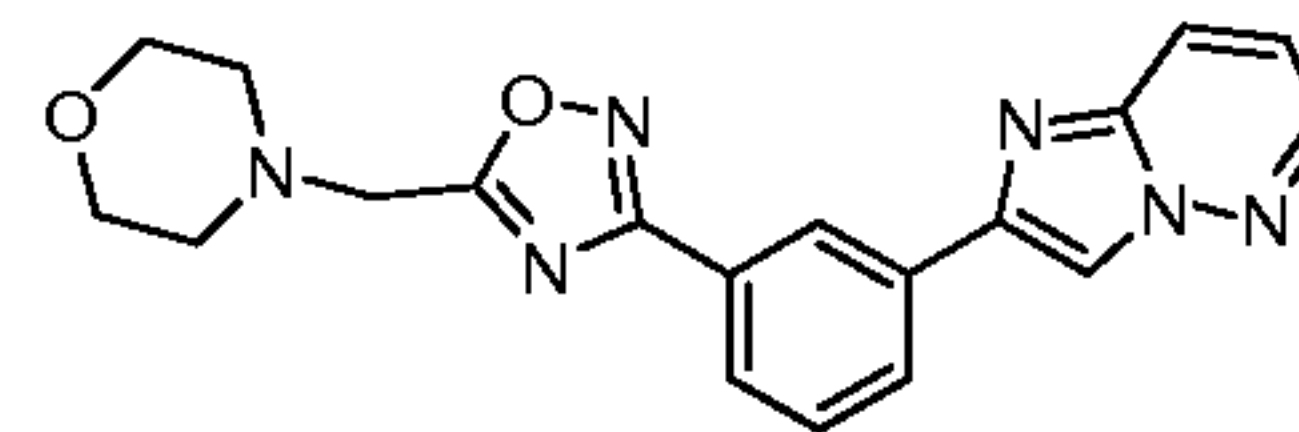
Compound 6
