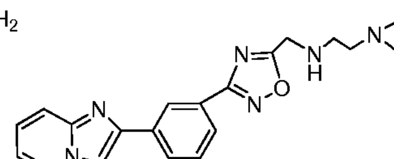
Compound 83
