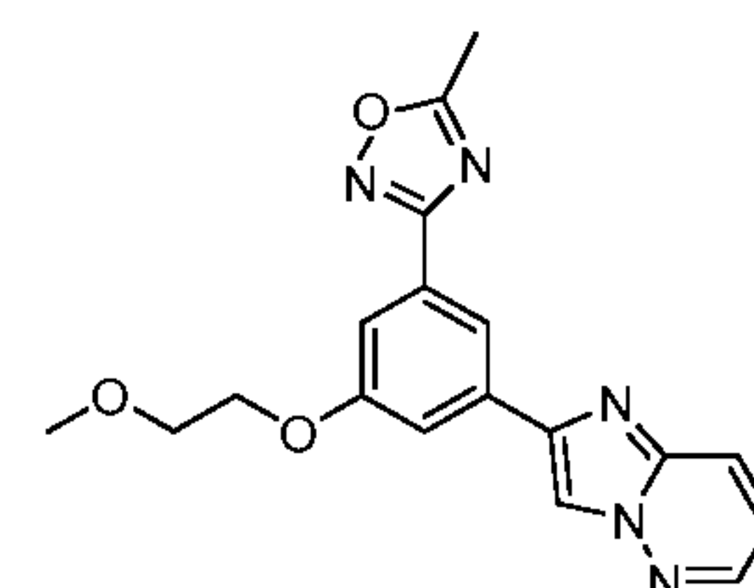
Compound 30
