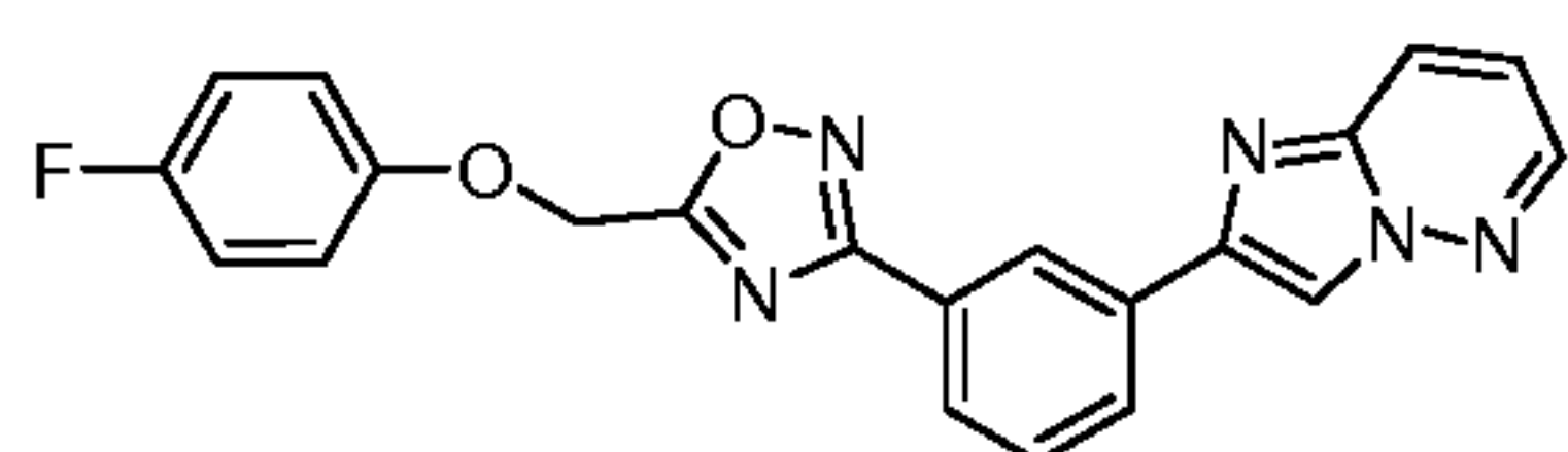
Compound 10
