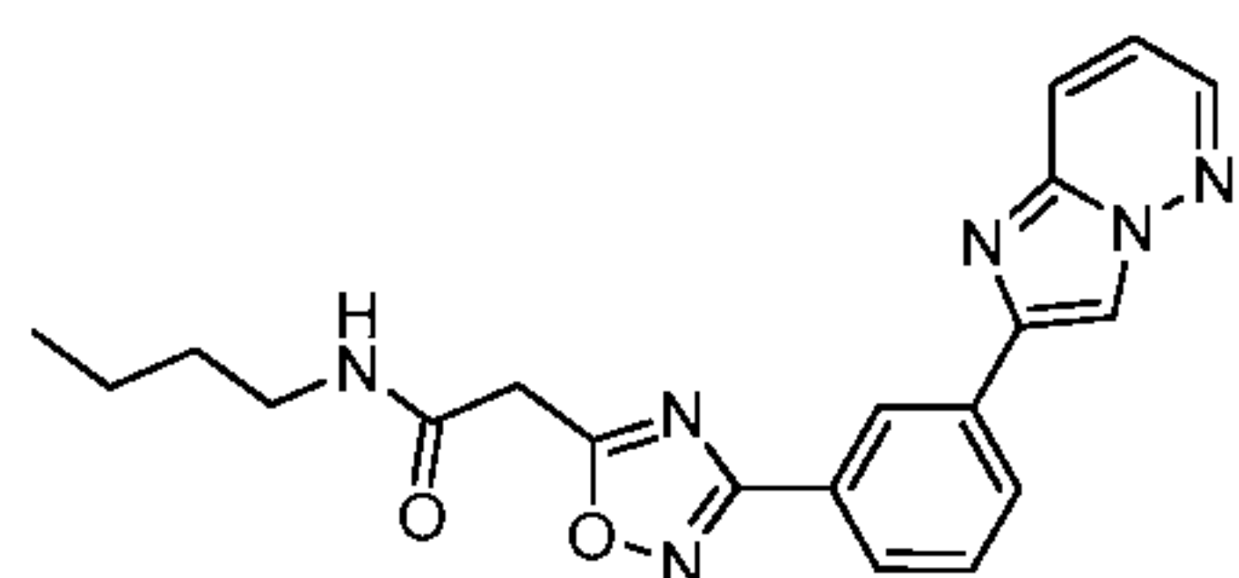
Compound 51
