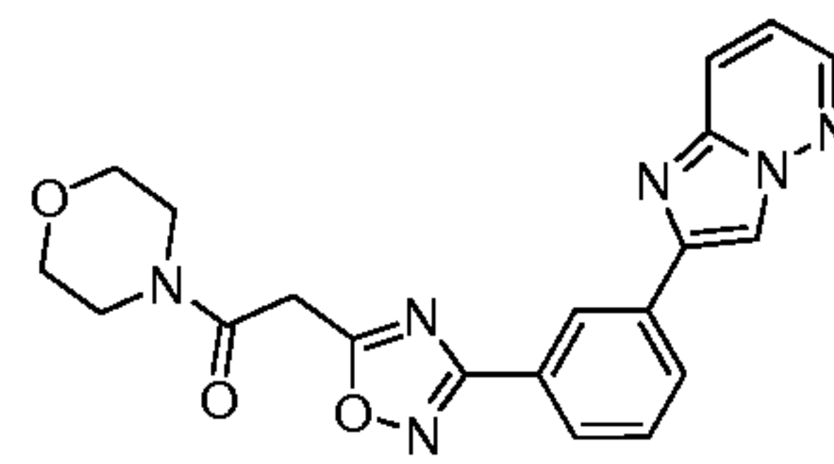
Compound 55
