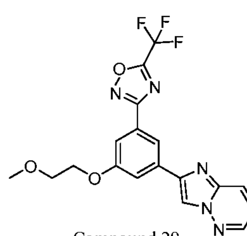
Compound 29
