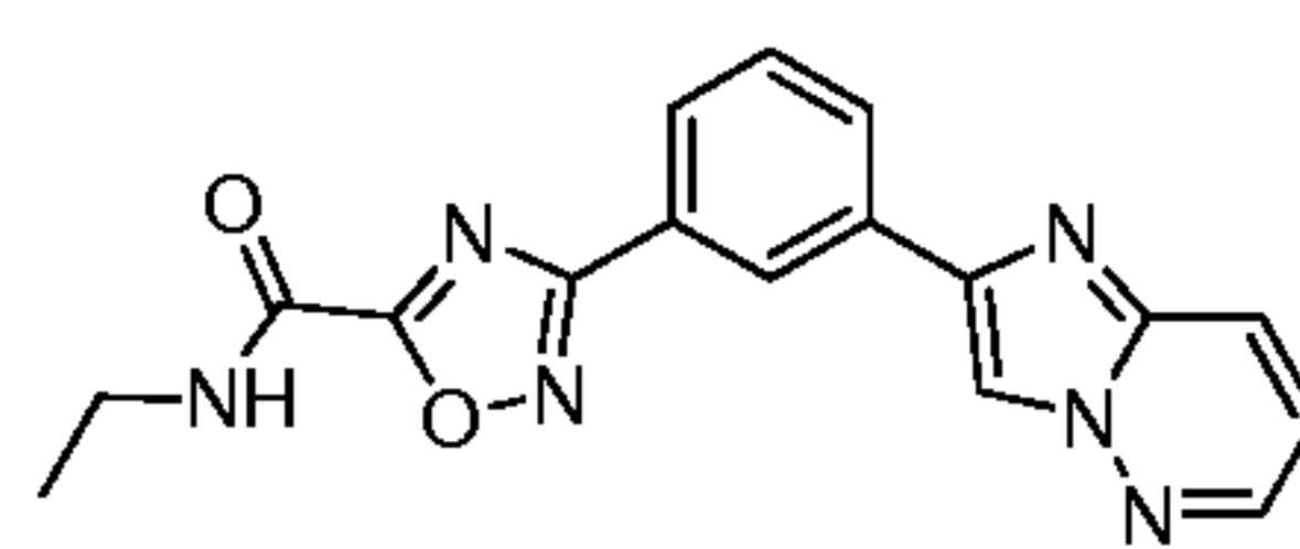
Compound 58
