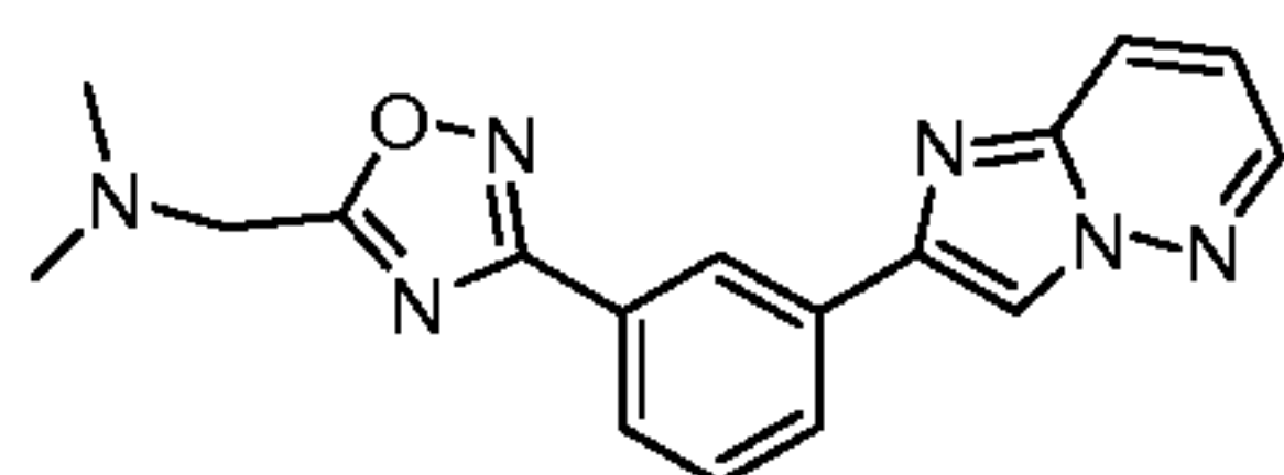
Compound 7
