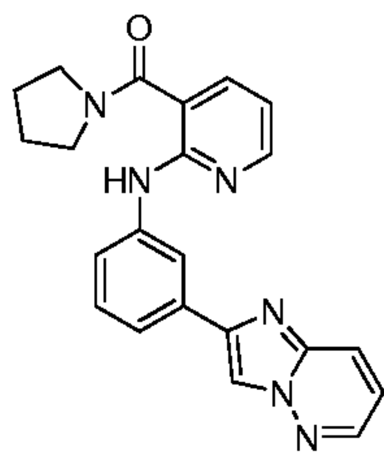
Compound 70
