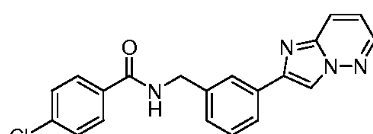
Compound 93
