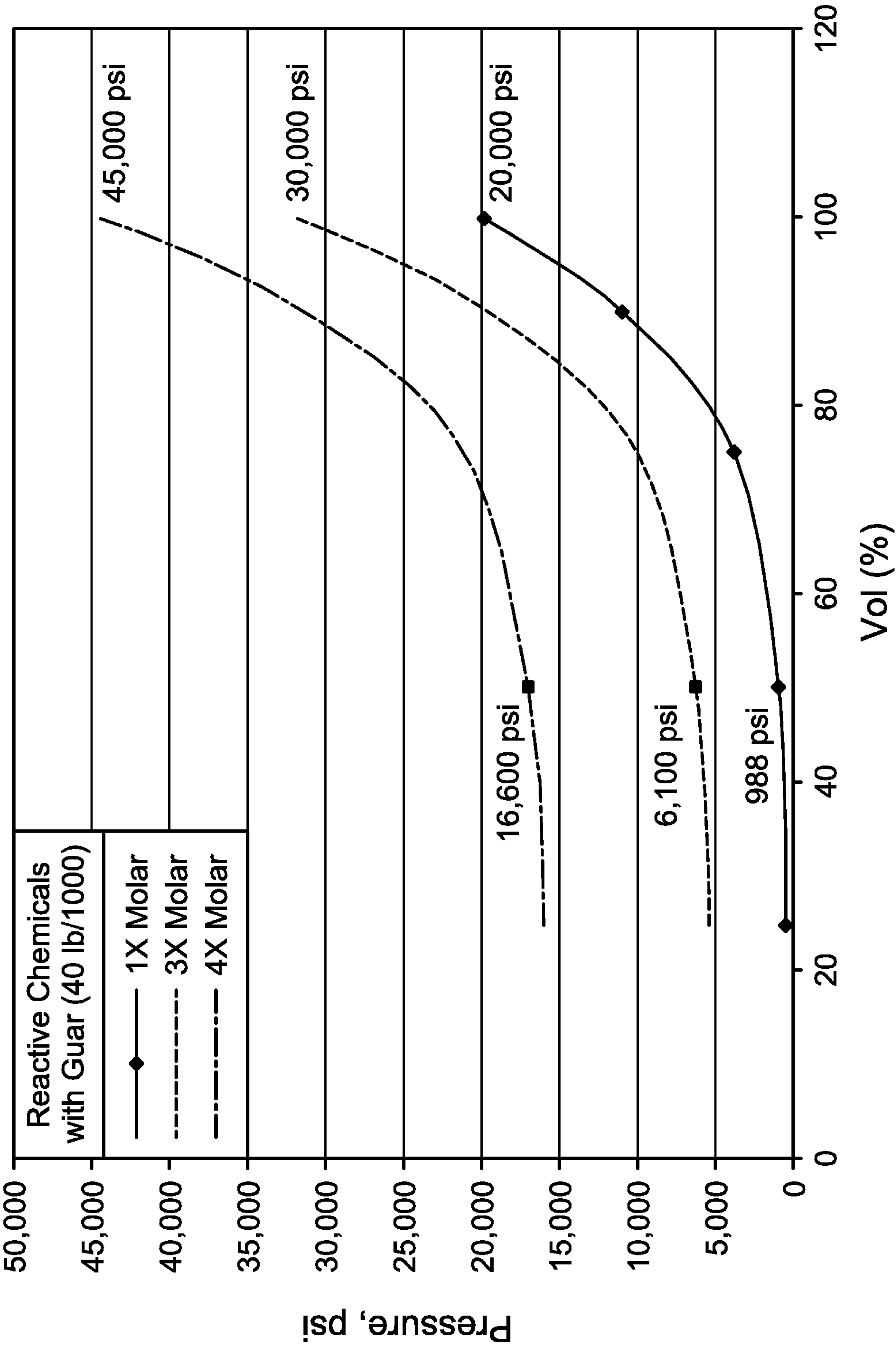
Autoclave Test of Redox at Different Molarity
