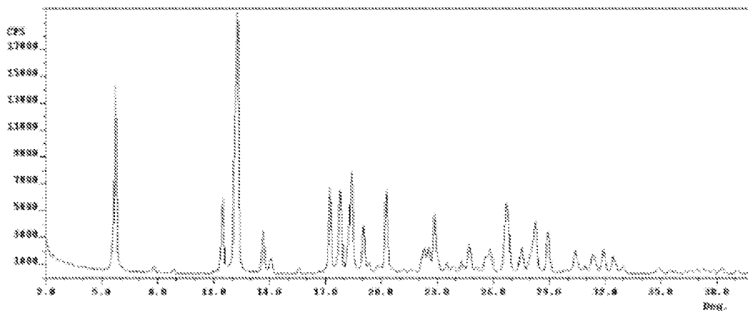
Fig.2: An X-ray powder diffraction pattern of crystalline pemetrexed diacid characterized by an X-ray powder diffraction pattern with peaks at about 5.7, 12.2, 17.2 and 18.4 degrees two-theta \pm 0.2 degrees two-theta.
