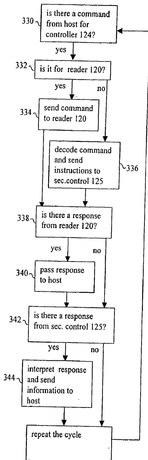
Fig. 3C General Process Summary
