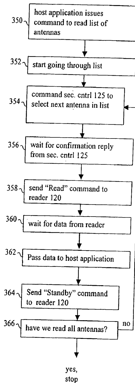
Fig. 3D Process for reading several antennas
