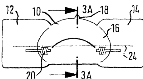
FIG. 3 PRIOR ART
