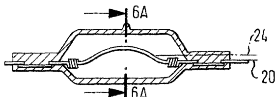
FIG. 6 PRIOR ART
