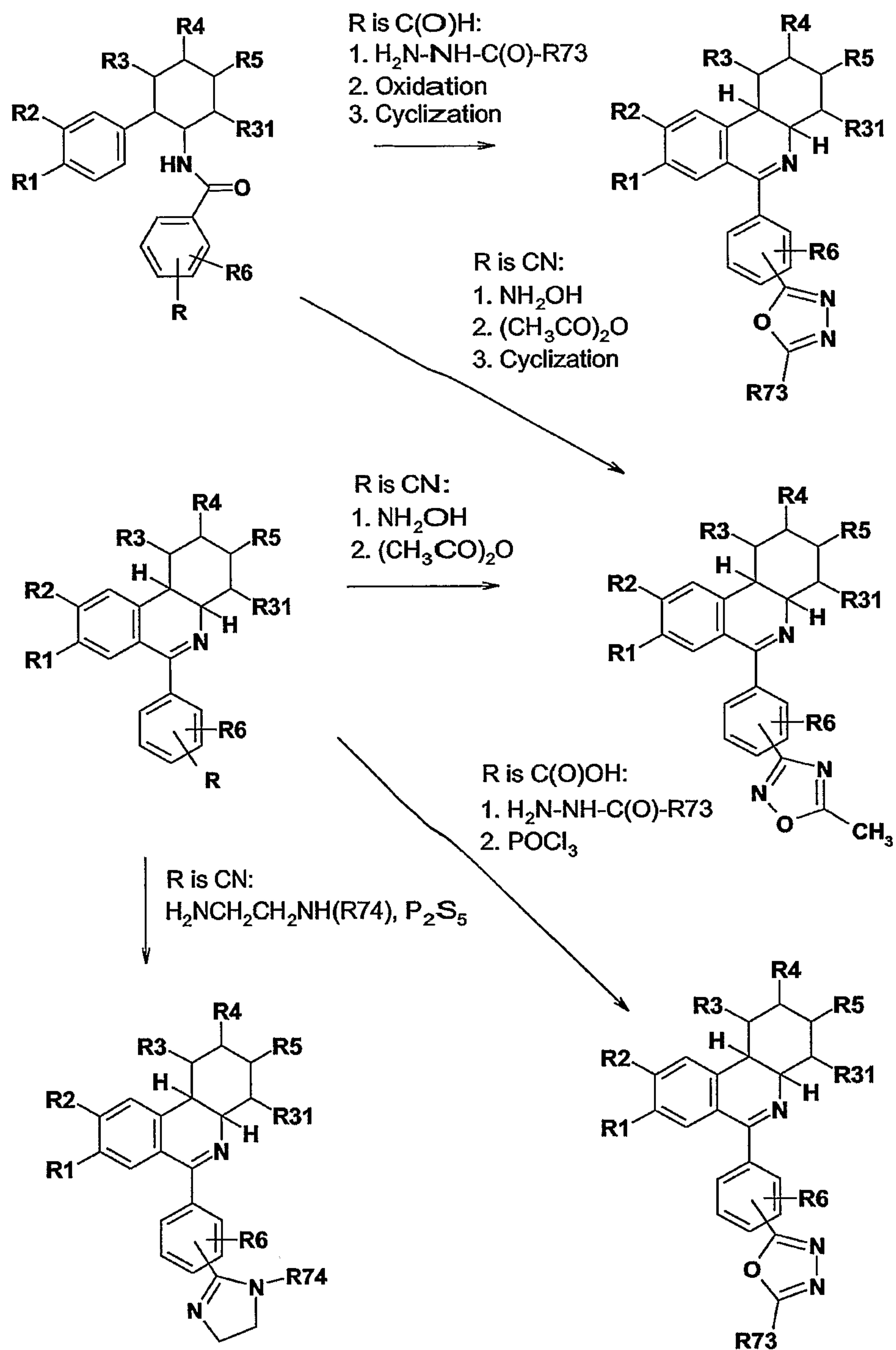
Reaction scheme 7:
