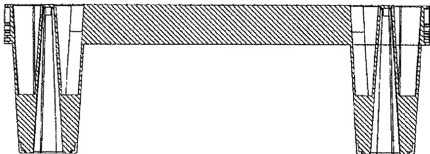
Fig. 82 Section C-C
