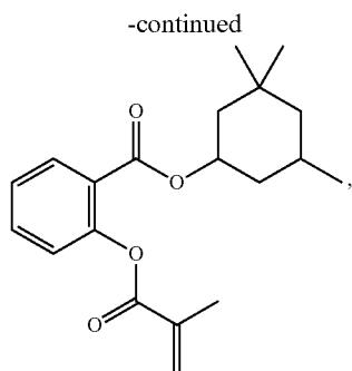
3,3,5-trimethylcyclohexyl 2-(methacryloxy)benzoate
