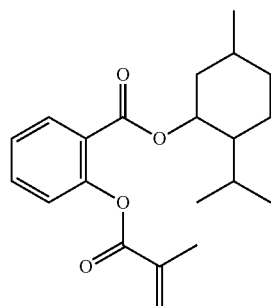
2-isopropyl-5-methylcyclohexyl 2-(methacryloxy)benzoate
