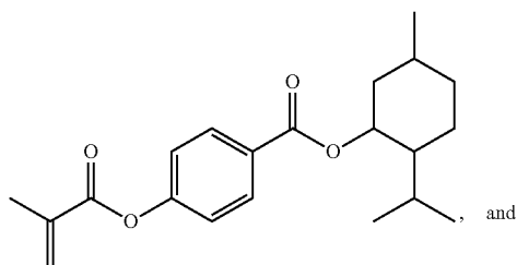
2-isopropyl-5-methylcyclohexyl 4-(methacryloxy)benzoate
