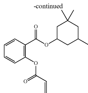
3,3,5-trimethylcyclohexyl 2-(acryloxy)benzoate
