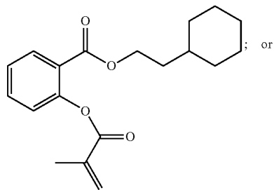
2-(methacryloyloxy)benzoic acid-2-cyclohexylethyl ester
