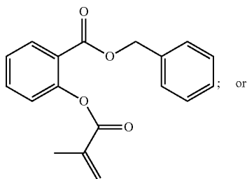
2-(methacryloyloxy)benzoic acid benzyl ester
