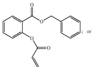
2-(acryloyloxy)benzoic acid benzyl ester
