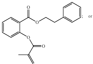
2-(methacryloyloxy)benzoic acid phenethyl ester
