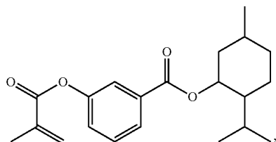
2-isopropyl-5-methylcyclohexyl 3-(methacryloxy)benzoate
