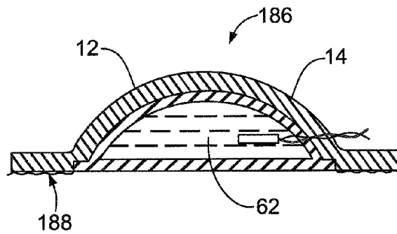
FIG. 4 (Prior Art)
