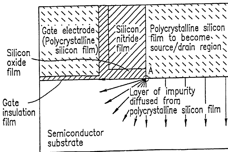
FIG. 12 Gate electrode lateral wall insulation film
