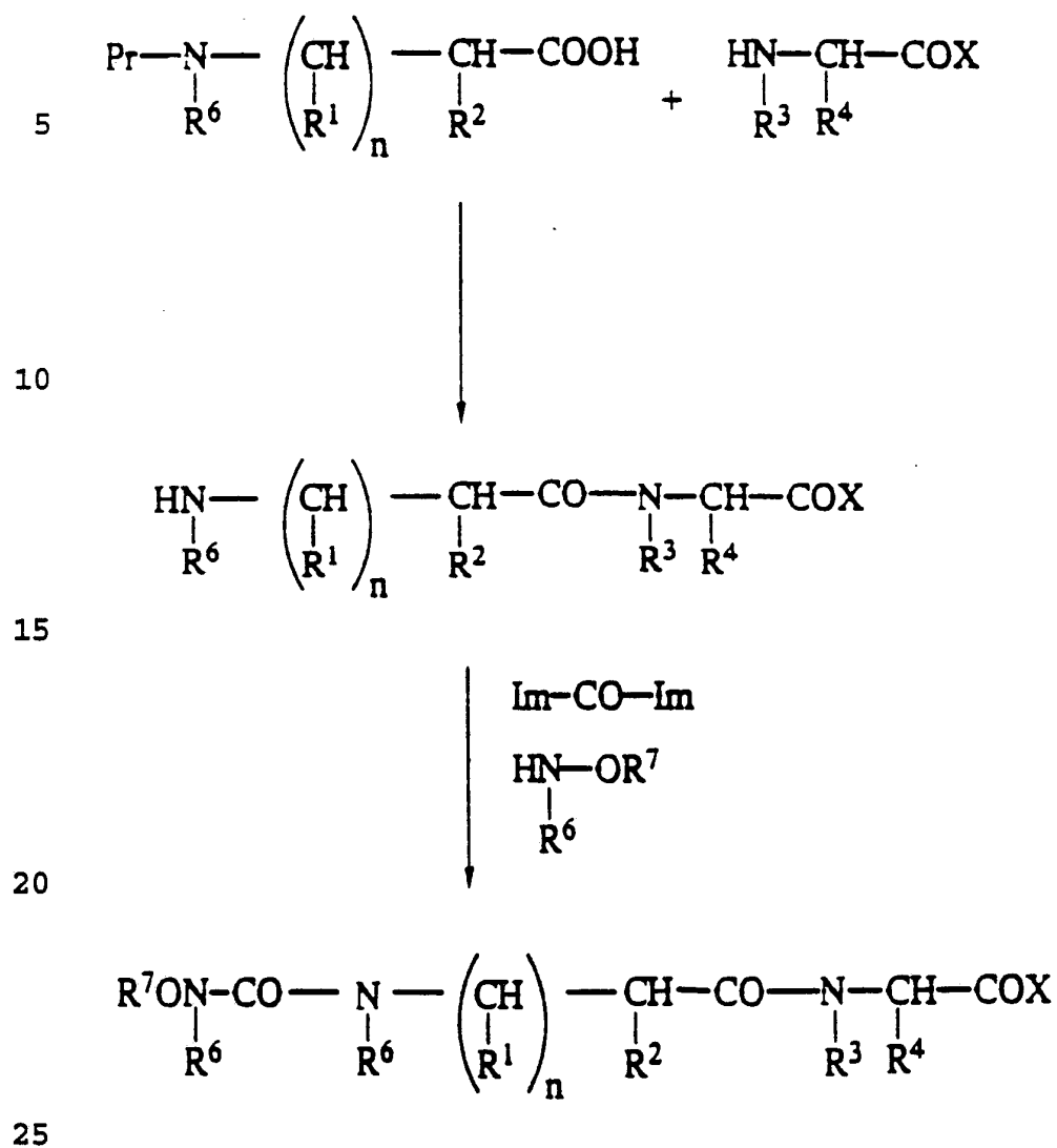
REACTION SCHEME 2
