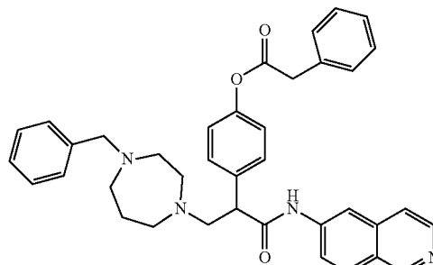
4-(3-(4-benzyl-1,4-diazepan-1-yl)-1-(isoquinolin-6-ylamino)-1-oxopropan-2-yl)phenyl 2-phenylacetate
