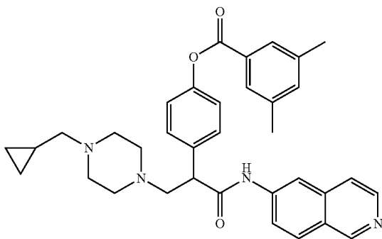
4-(3-(4-(cyclopropylmethyl)piperazin-1-yl)-1-(isoquinolin-6-ylamino)-1-oxopropan-2-yl)phenyl 3,5-dimethylbenzoate
