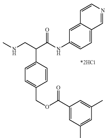
4-(1-(isoquinolin-6-ylamino)-3-(methylamino)-1-oxopropan-2-yl)benzyl 3,5-dimethylbenzoate
