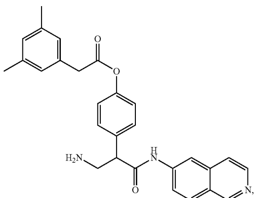
4-(3-amino-1-(isoquinolin-6-ylamino)-1-oxopropan-2-yl)phenyl 2-(3,5-dimethylphenyl)acetate
