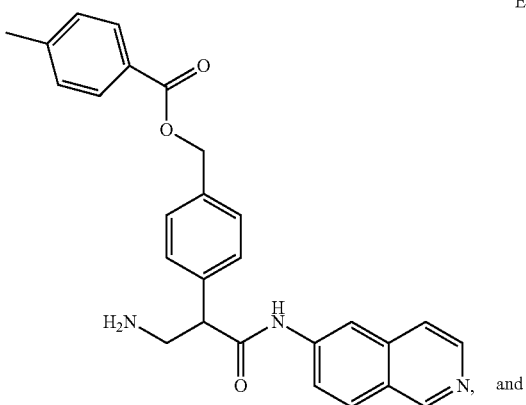
4-(3-amino-1-(isoquinolin-6-ylamino)-1-oxopropan-2-yl)benzyl 4-methylbenzoate
