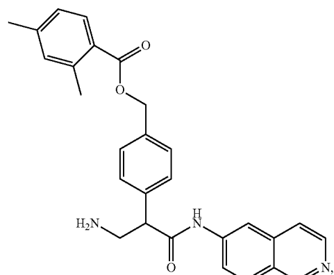
4-(3-amino-1-(isoquinolin-6-ylamino)-1-oxopropan-2-yl)benzyl 2,4-dimethylbenzoate
