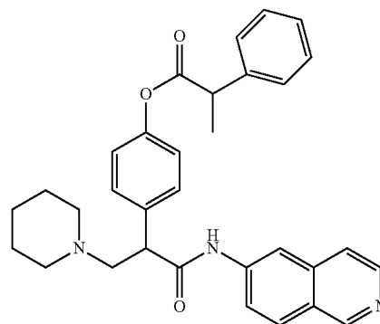
4-(1-(isoquinolin-6-ylamino)-1-oxo-3-(piperidin-1-yl)propan-2-yl)phenyl 2-phenylpropanoate
