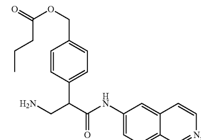
4-(3-amino-1-(isoquinolin-6-ylamino)-1-oxopropan-2-yl)benzyl butyrate
