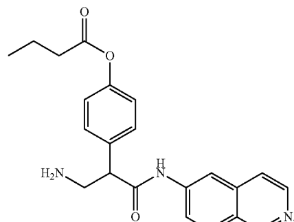
4-(3-amino-1-(isoquinolin-6-ylamino)-1-oxopropan-2-yl)phenyl butyrate
