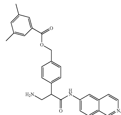
4-(3-amino-1-(isoquinolin-6-ylamino)-1-oxopropan-2-yl)benzyl 3,5-dimethylbenzoate
