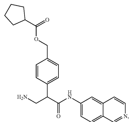
4-(3-amino-1-(isoquinolin-6-ylamino)-1-oxopropan-2-yl)benzyl cyclopentanecarboxylate
