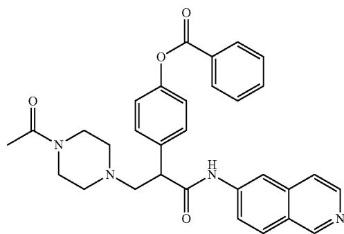
4-(3-(4-acetylpiperazin-1-yl)-1-(isoquinolin-6-ylamino)-1-oxopropan-2-yl)phenyl benzoate
