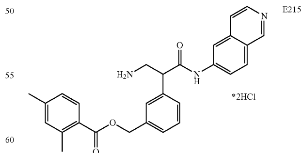
3-(3-amino-1-(isoquinolin-6-ylamino)-1-oxopropan-2-yl)benzyl 2,4-dimethylbenzoate
