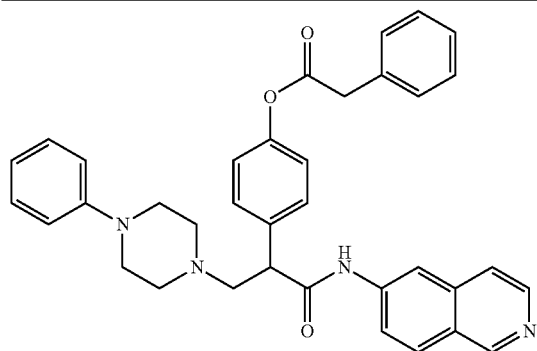
4-(1-(isoquinolin-6-ylamino)-1-oxo-3-(4-phenylpiperazin-1-yl)propan-2-yl)phenyl 2-phenylacetate
