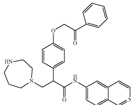
3-(1,4-diazepan-1-yl)-N-(isoquinolin-6-yl)-2-(4-(2-oxo-2-phenylethoxy)phenyl)propanamide
