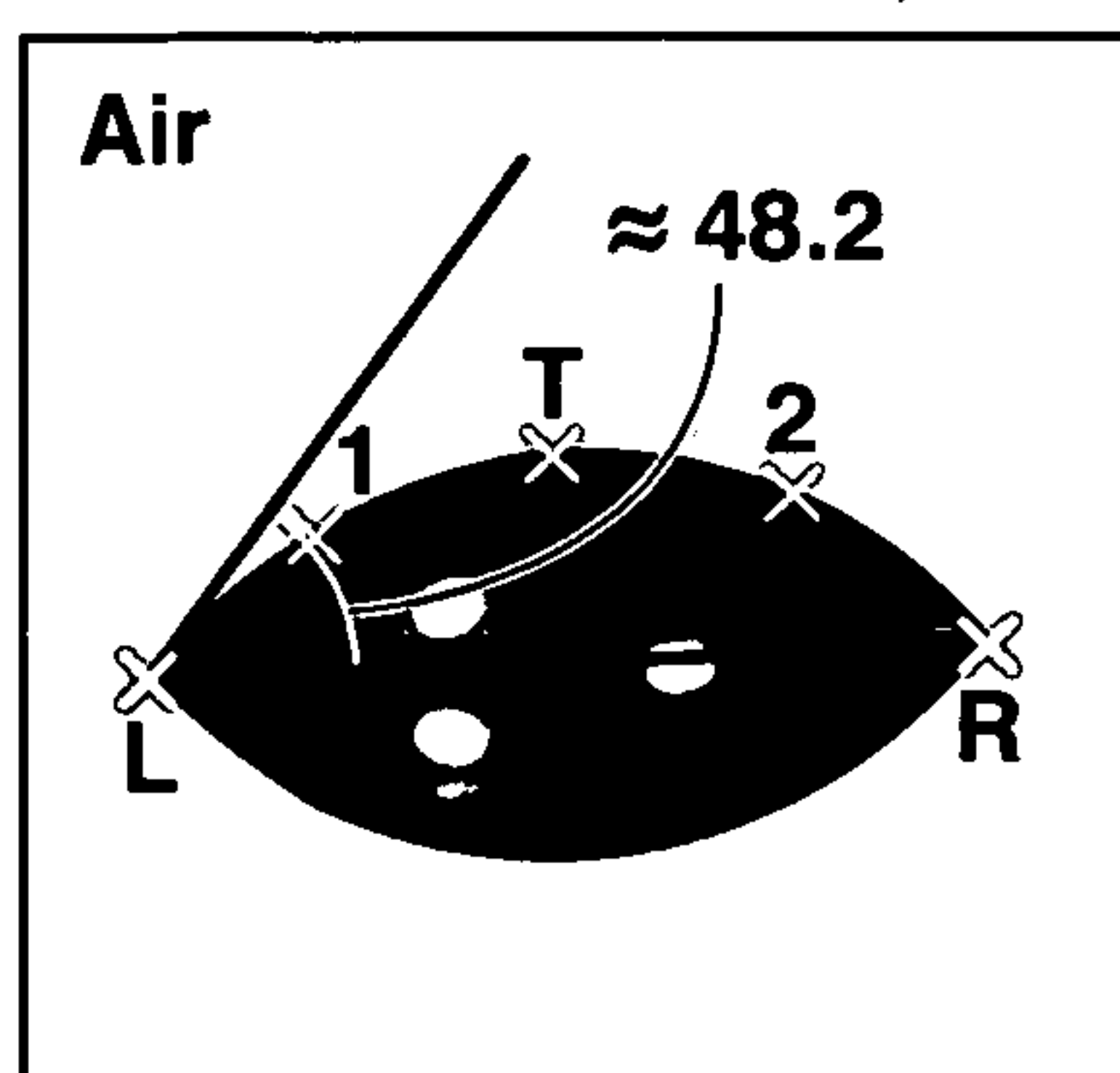
Uncoated 4142 Steel
