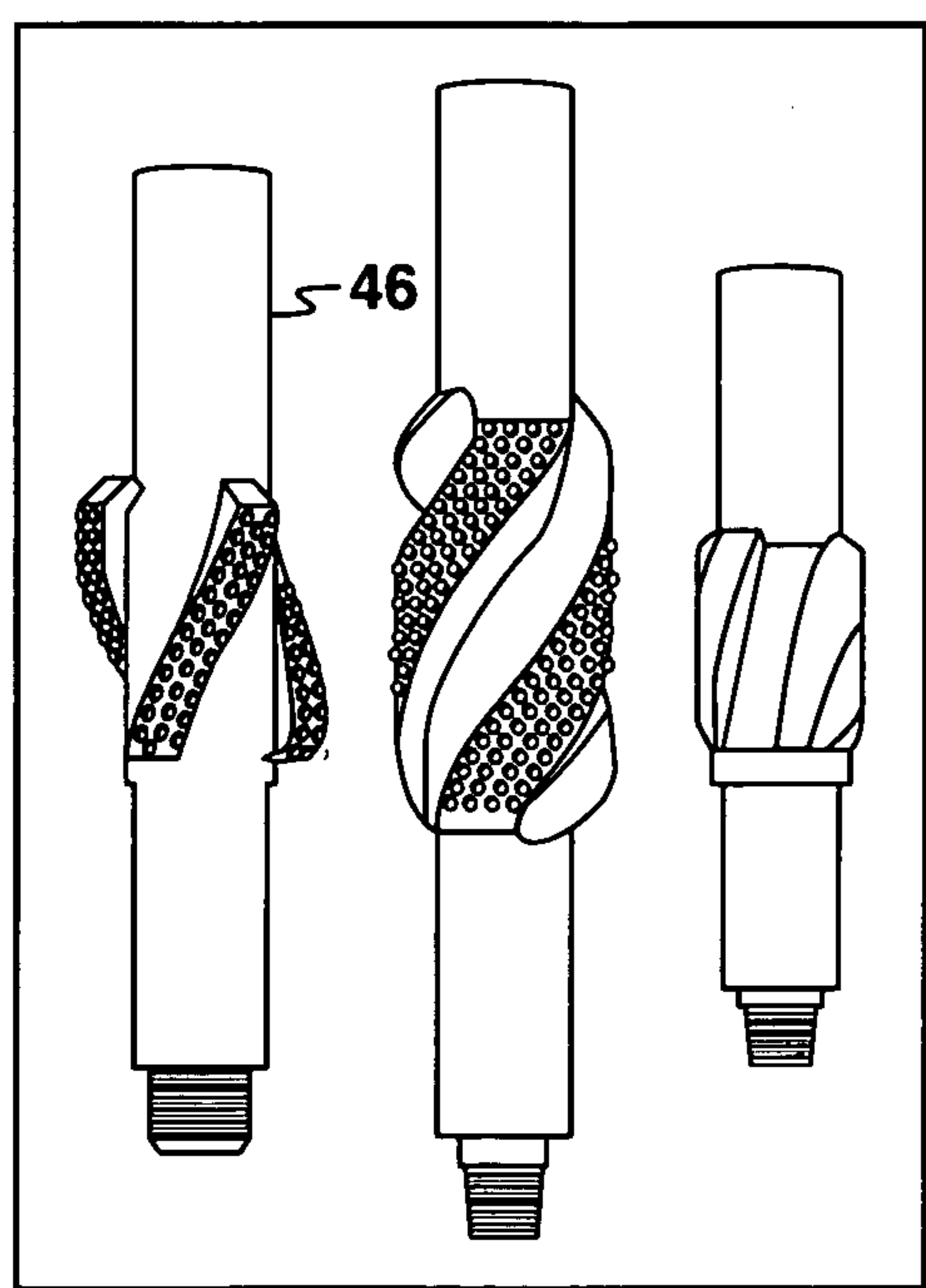
FIG. 3D
