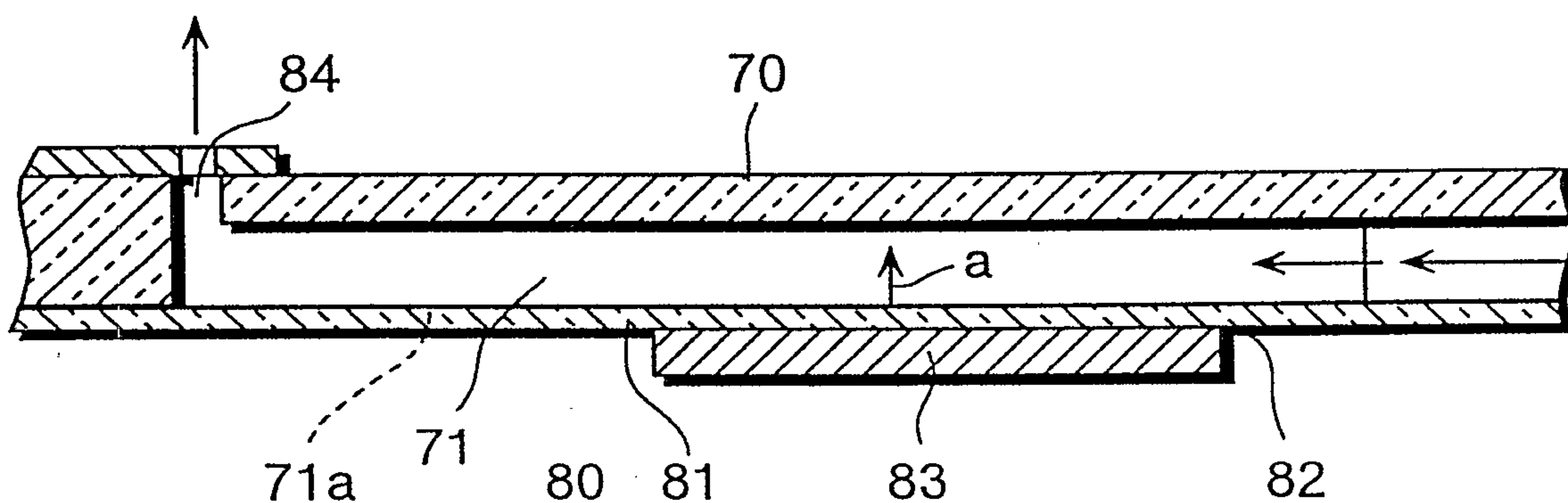
Fig.17 Prior Art
