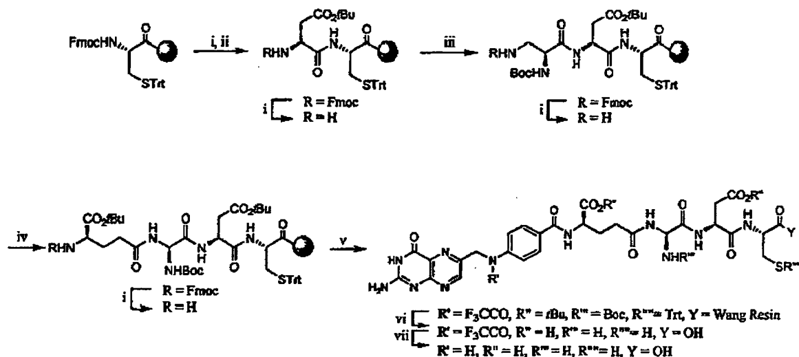
Scheme 1 a
