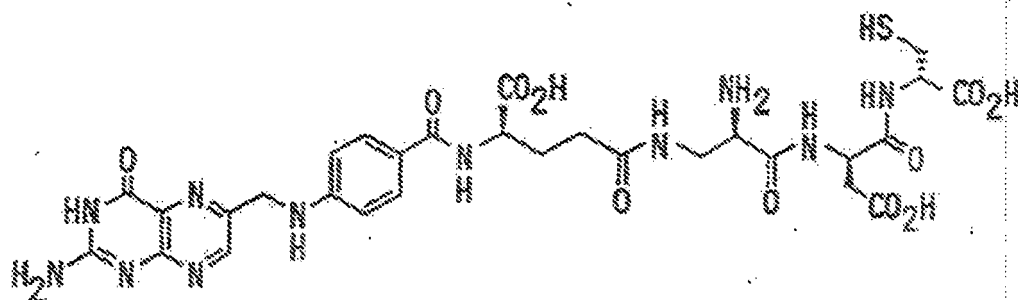
EC53 (Pte-D-γGlu-D-βDpr-D-Asp-D-Cys)
