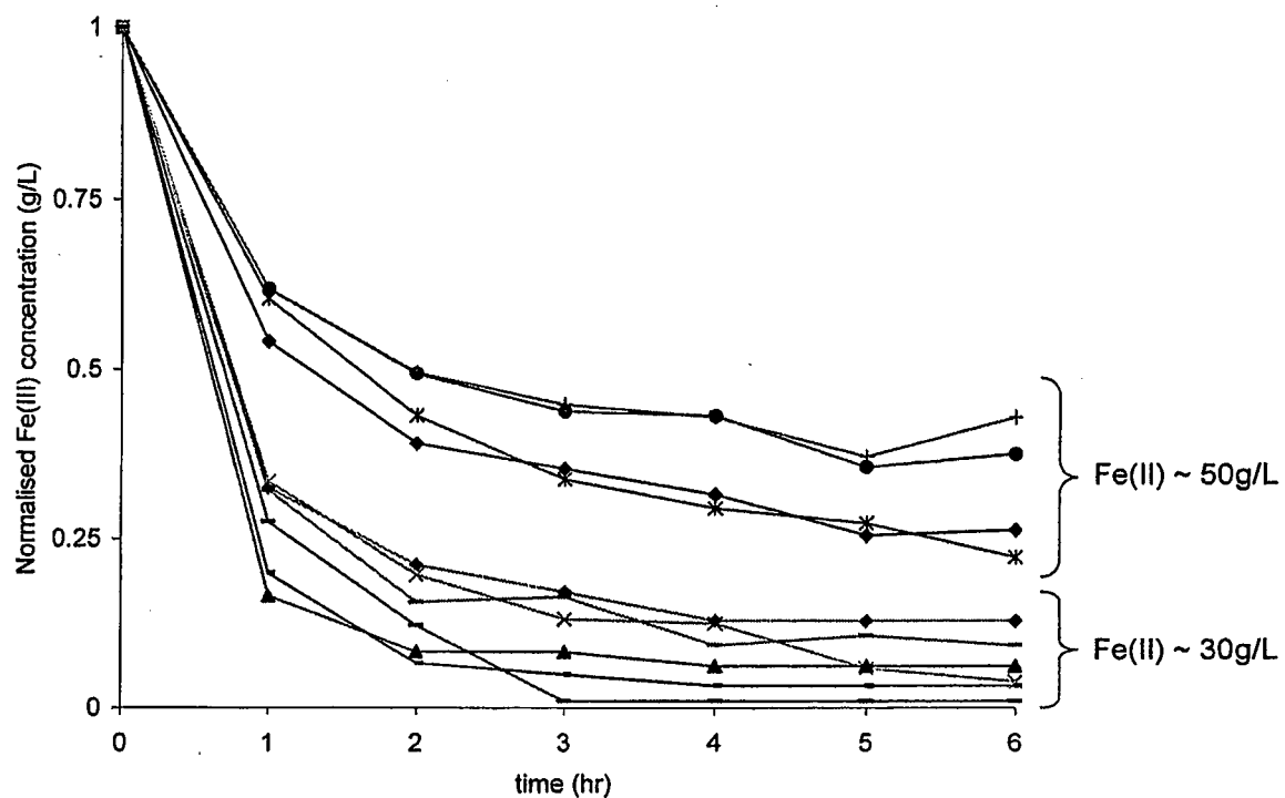
Figure 3: Overlaid graphs of the decrease in Fe(III) concentration with time the solution/ catalyst contact time. Two distinct sections of this graph can be observed showing a marked dependence on Fe(II) concentration.
