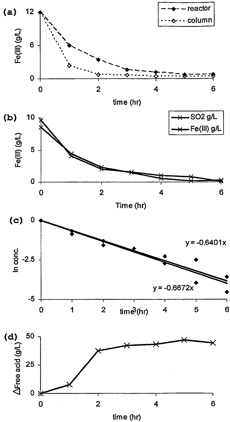
Figure 2: A series of graphs obtained from each SO 2 -Fe(III) reduction experimental run in Example 1.
