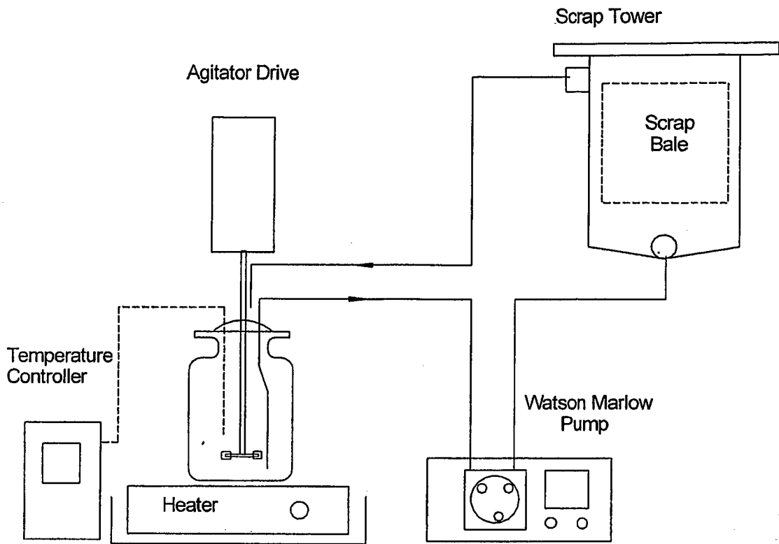
Figure 4 - Iron Reduction Experimental Set Up for Example 2
