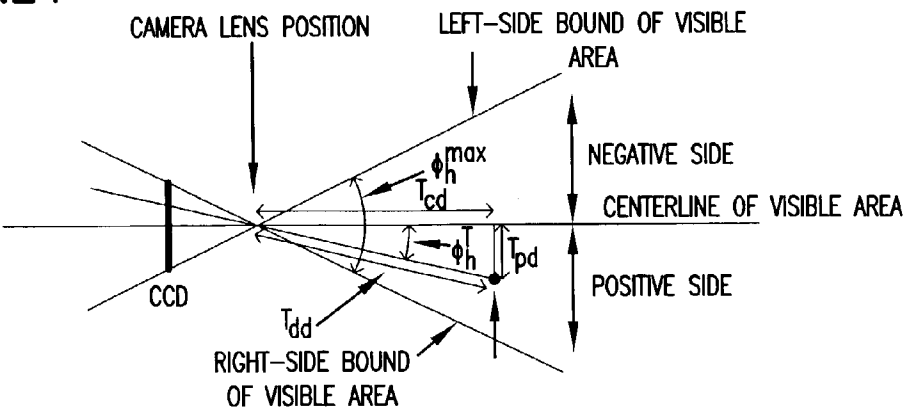
TOP VIEW OF GEOMEYTLICAL RELATION
