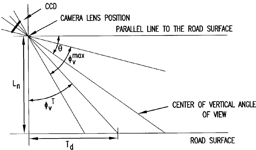
SIDE VIEW OF GEOMETRICAL RELATION
