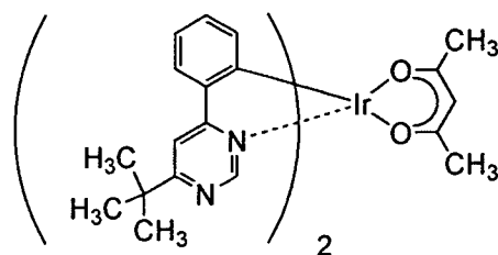
[\text{Ir}(\text{tBuppm})_2(\text{acac})]
