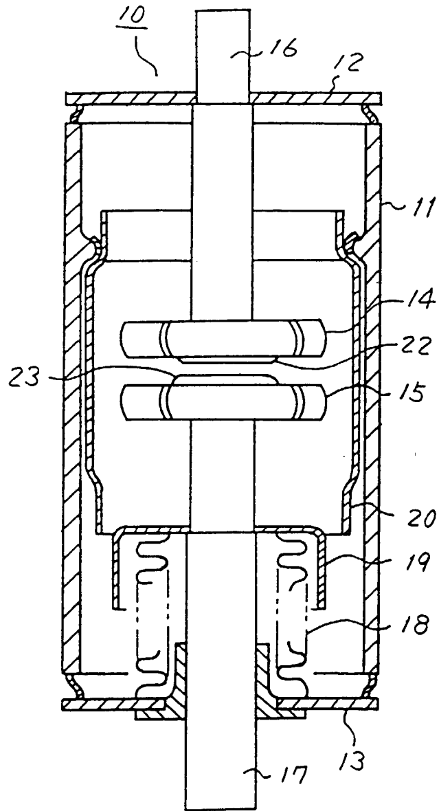
FIG. 10 (PRIOR ART)
