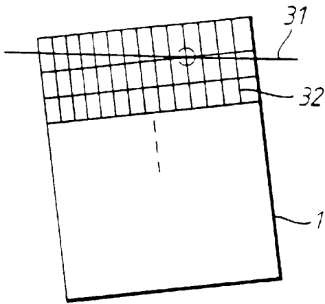
Fig. 4 (PRIOR ART)
