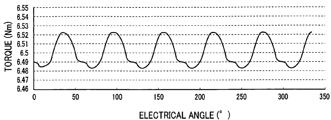
FIG. 12A (PRIOR ART)
