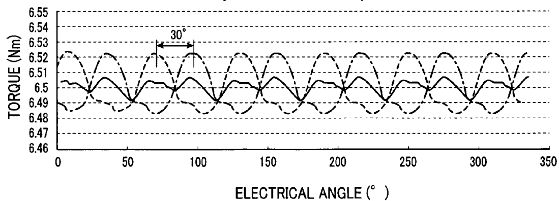
FIG. 12B (PRIOR ART)
