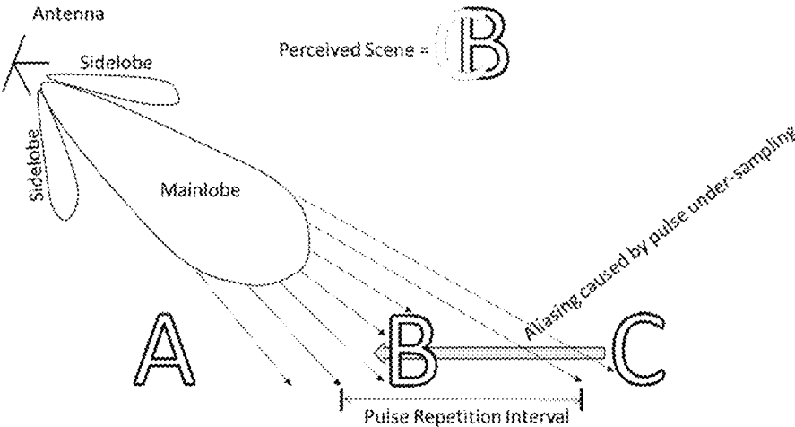
Radar Ambiguity Illustration
