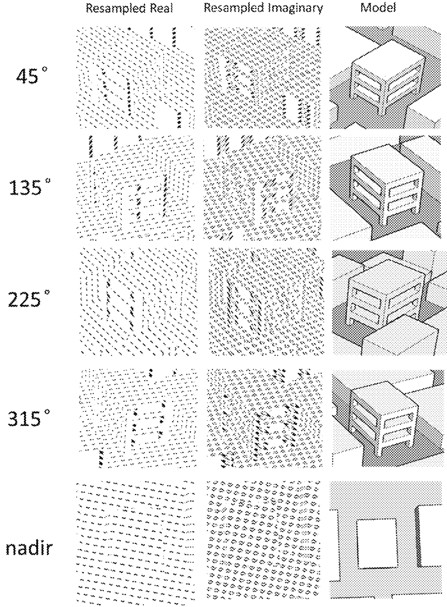
Complex resampling illustration for model parking structure
