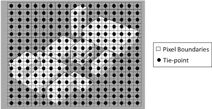
Focal plane tie-point grid
