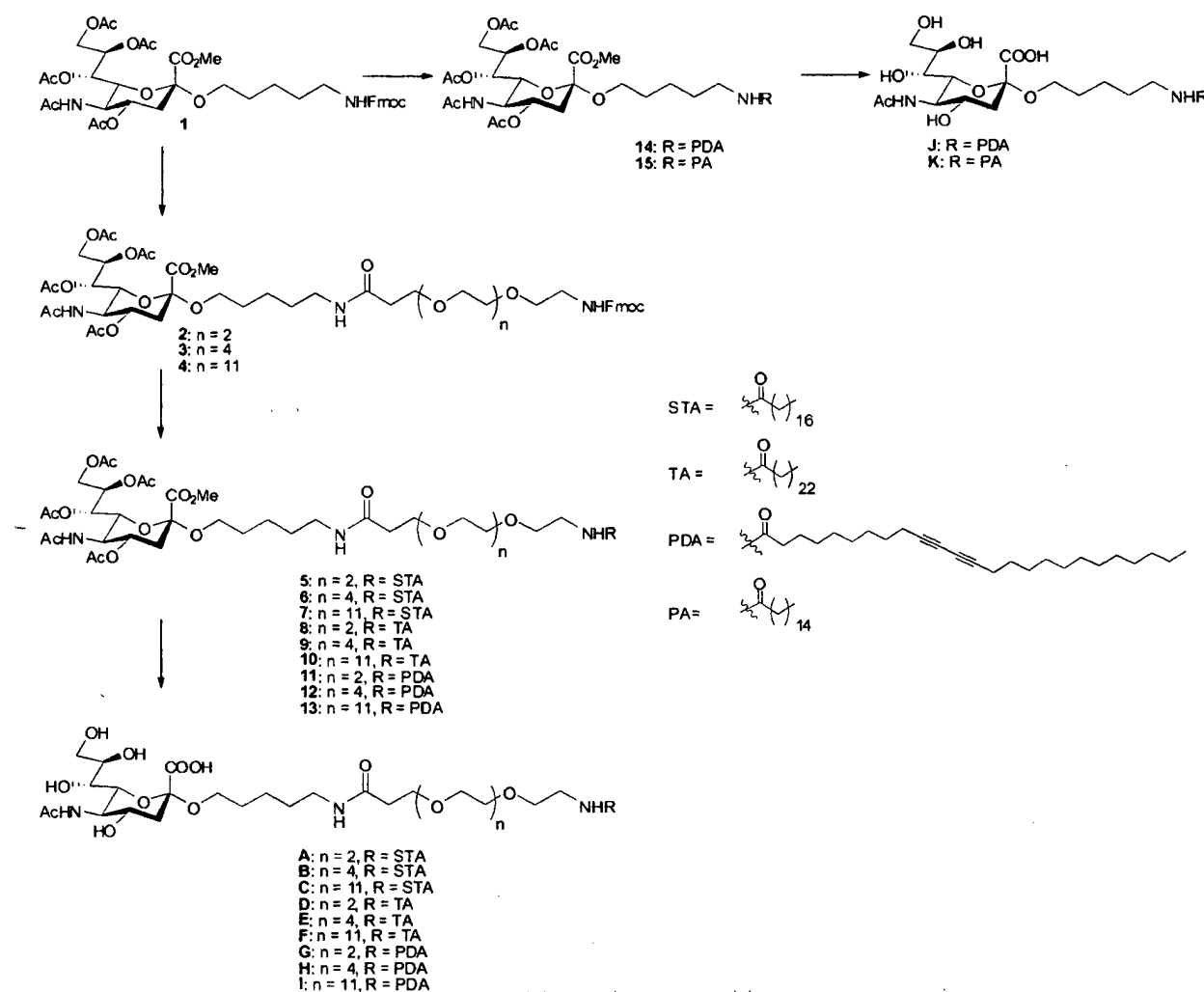
Scheme 1 Synthesis of compound A to K
