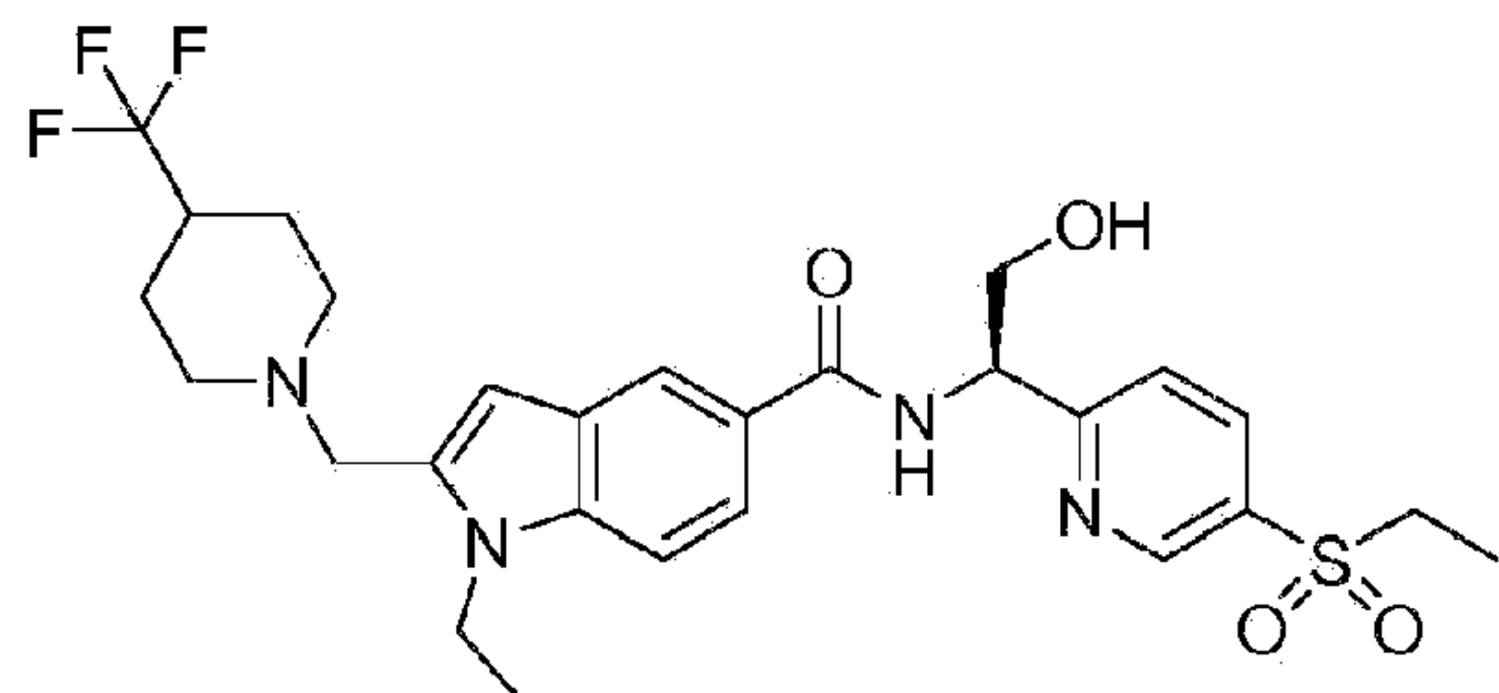
Compound IN-11
