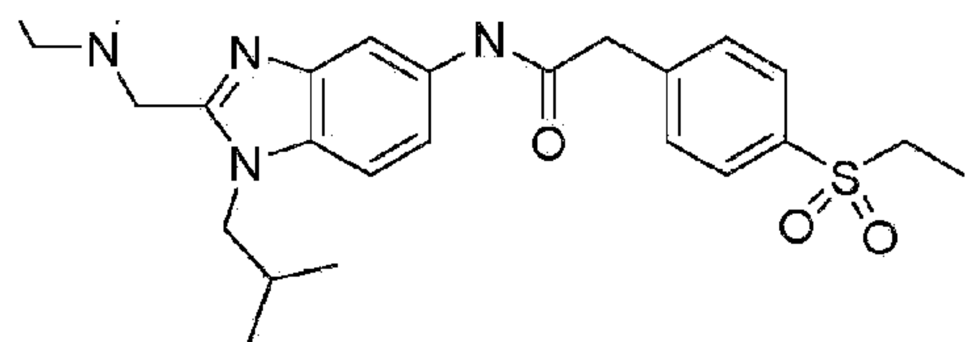
Compound BE-69
