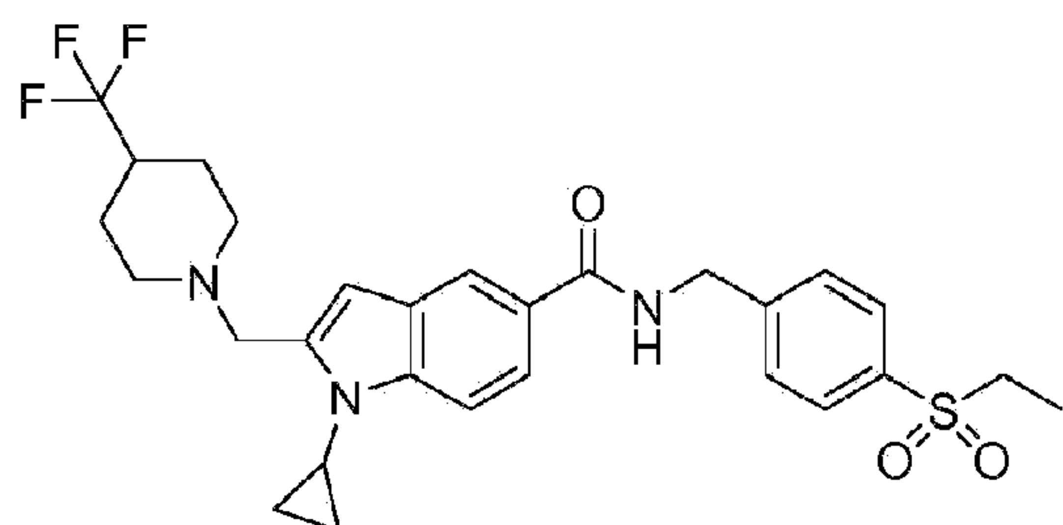
Compound IN-12
