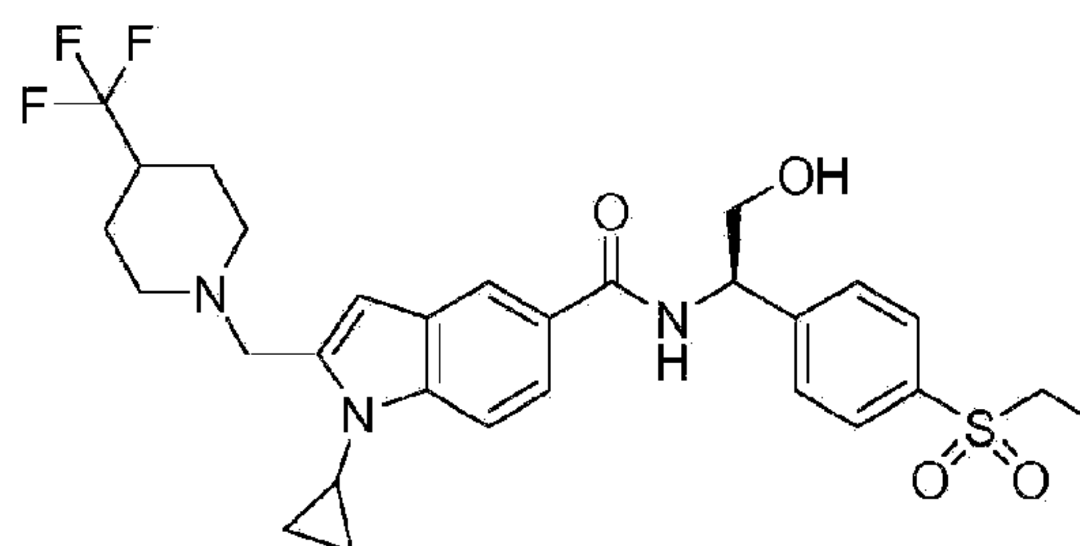
Compound IN-13
