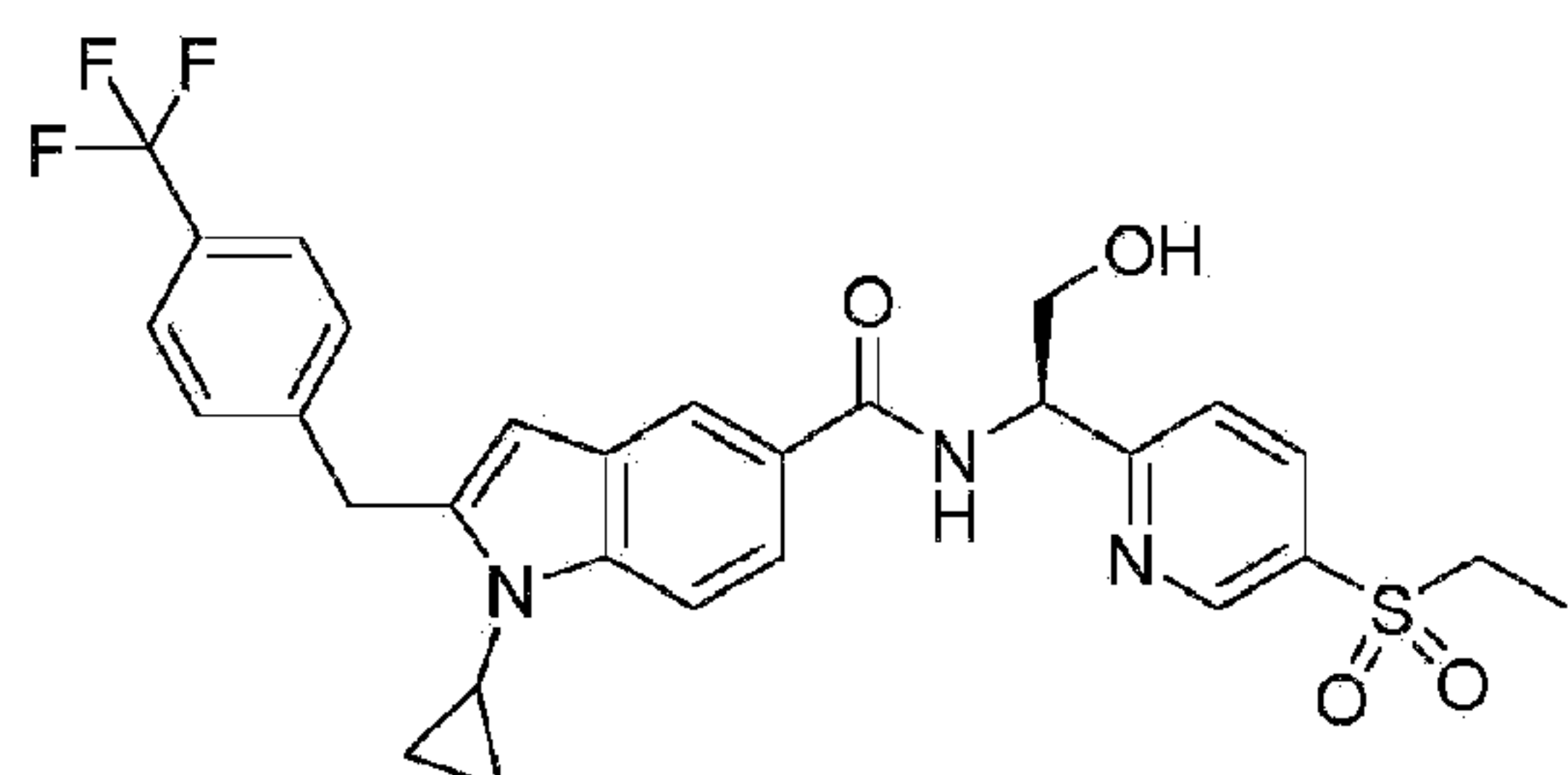
Compound IN-19
