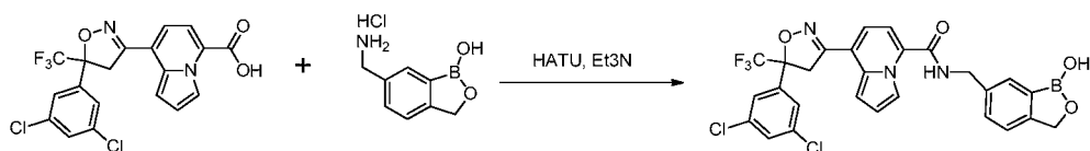
37a. 5-(5-(3,5-dichlorophenyl)-5-(trifluoromethyl)-4,5-dihydroisoxazol-3-yl)-N-((1-hydroxy-3,3-dimethyl-1,3-dihydrobenzo[c][1,2]oxaborol-6-yl)methyl)-N-methylindolizine-8-carboxamide
