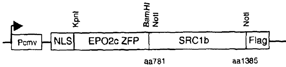
pSRC1b-EPO2c
