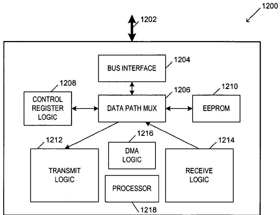
FIG. 12 (Prior Art)
