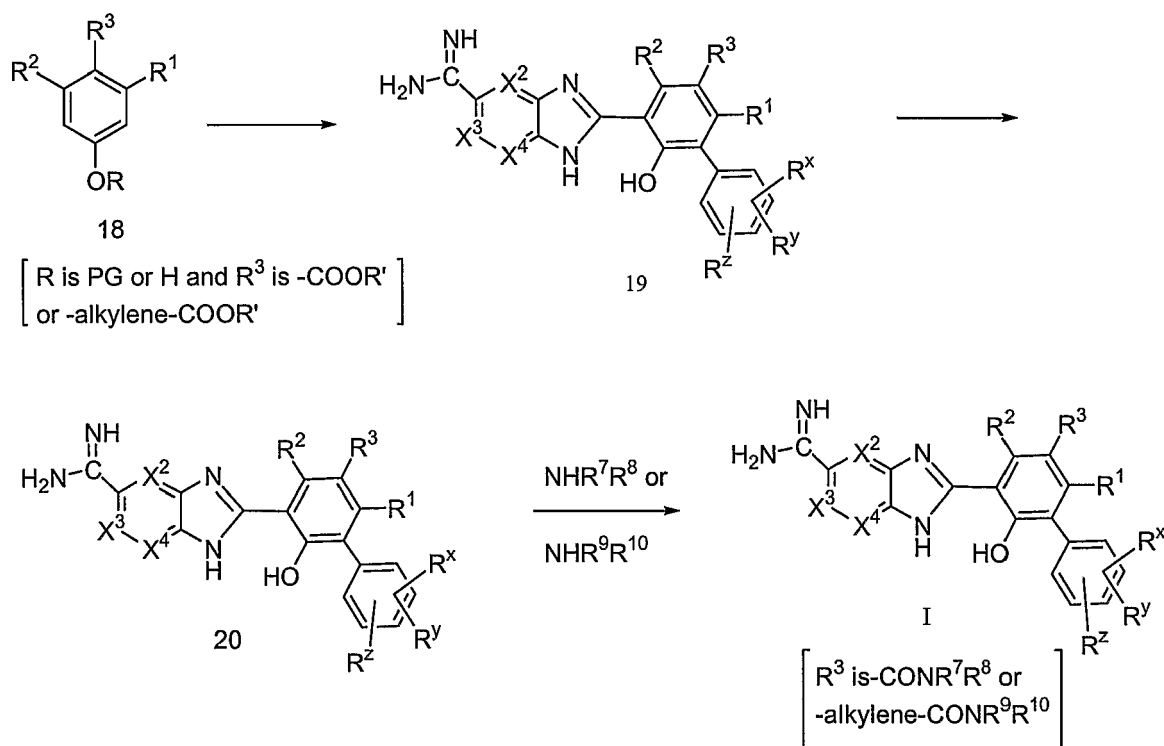
Scheme III
