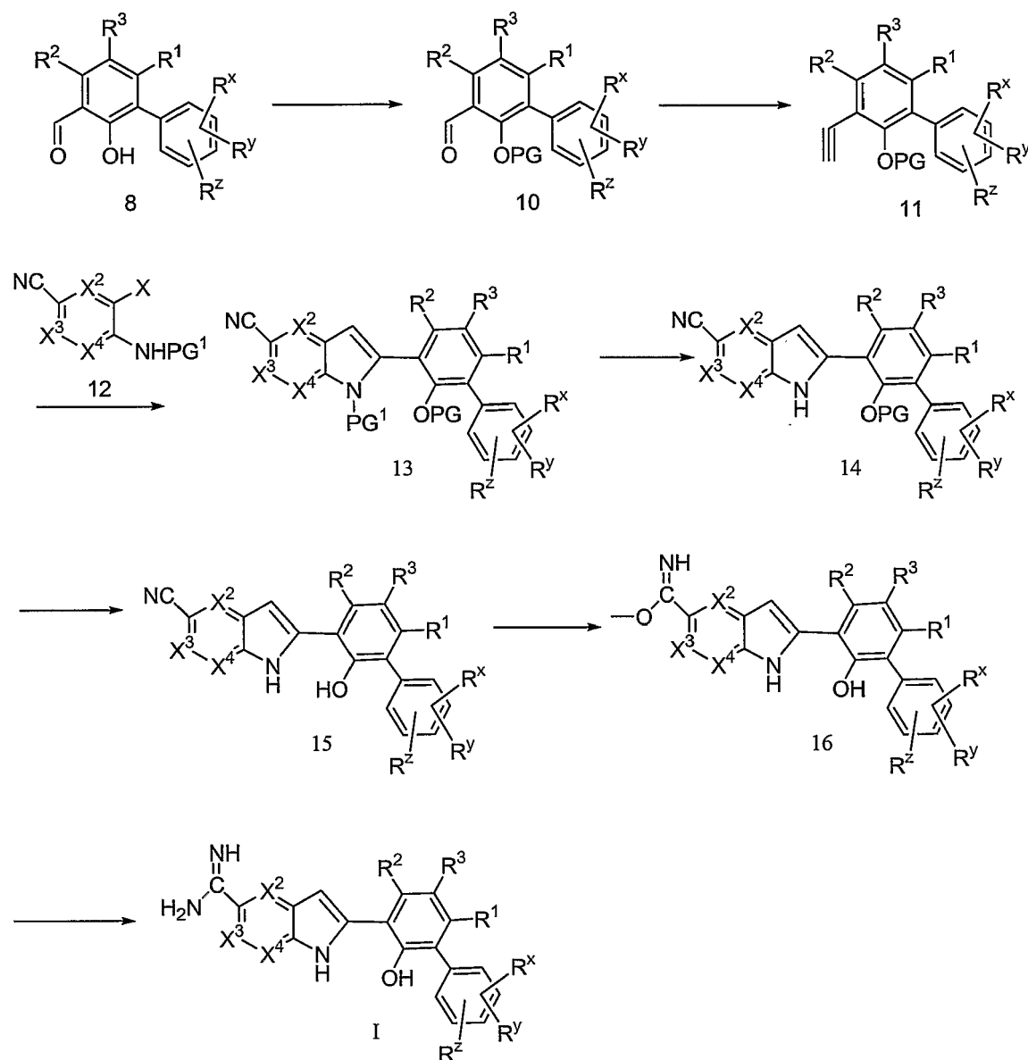
Scheme II
