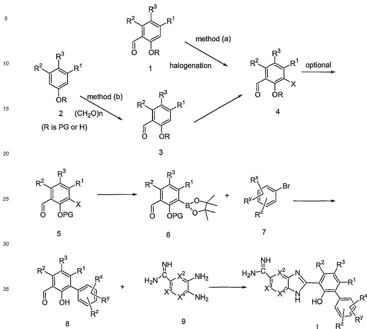
Scheme I
