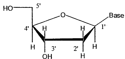
2'-deoxynucleoside
