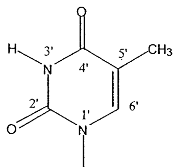
2'-deoxythymidine
