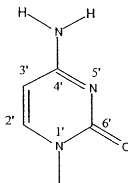
2'-deoxycytidine
