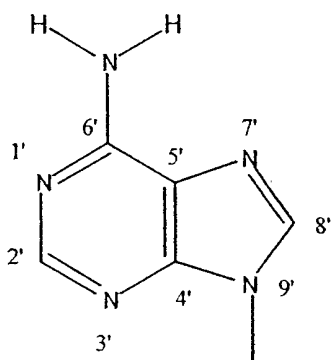
2'-deoxyadenosine
