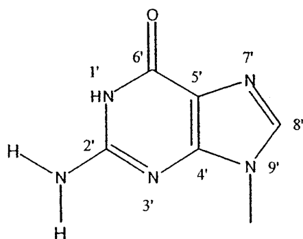
2'-deoxyguanosine
