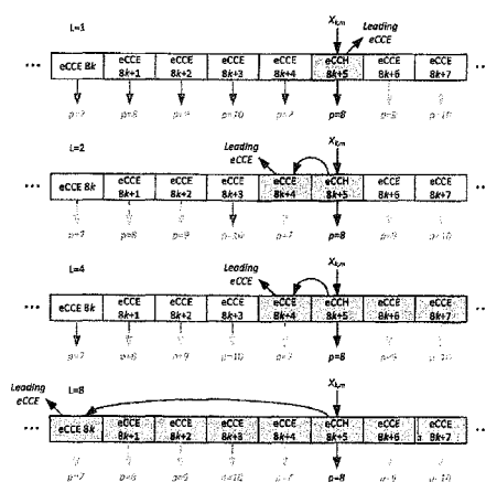
Figure 9: An Example of the Decision of the Leading eCCE and the DMRS port
