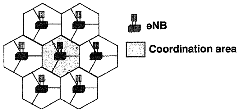
Figure 5 Scenario 1 - Homogeneous network with intra-site CoMP
