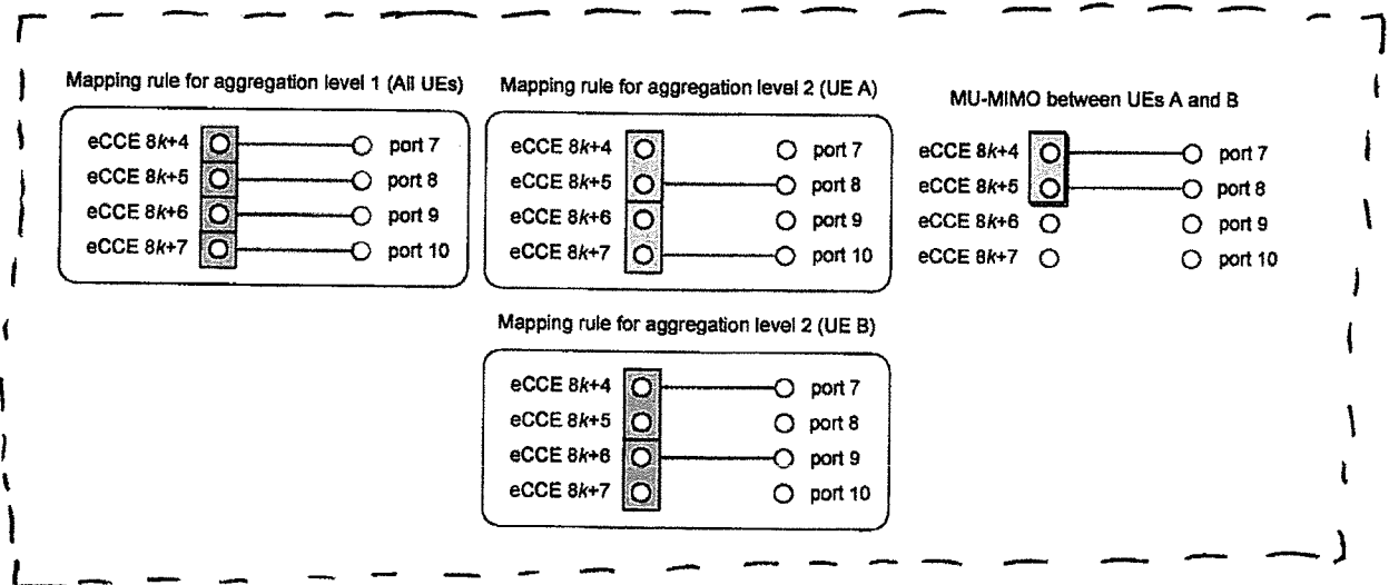
Figure 10 Example of DMRS port linkage
