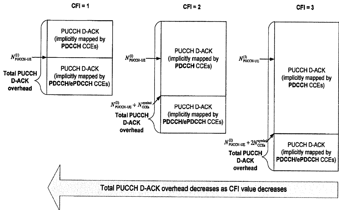
Figure 12 PUCCH D-ACK region implicitly mapped by ePDCCH CCEs (or eCCEs) changes depending on the value of CFI
