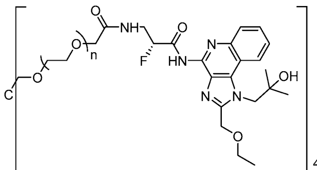
Compound 4
