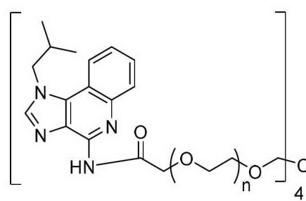
Compound 14
