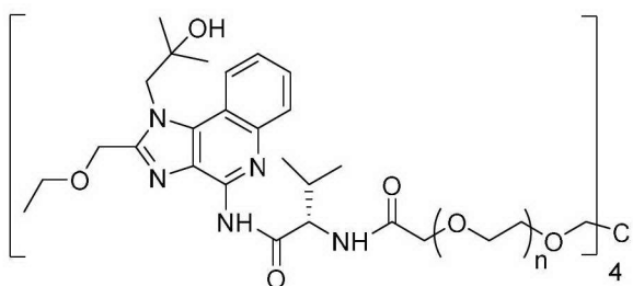
Compound 8
