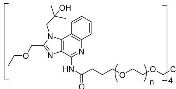
Compound 3
