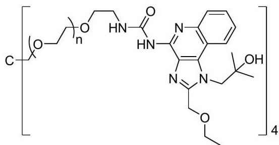
Compound 13
