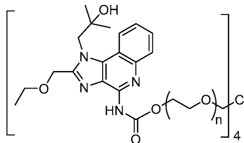
Compound 12
