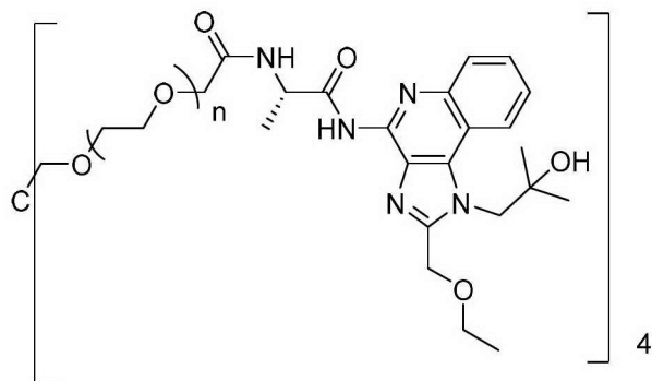
Compound 7
