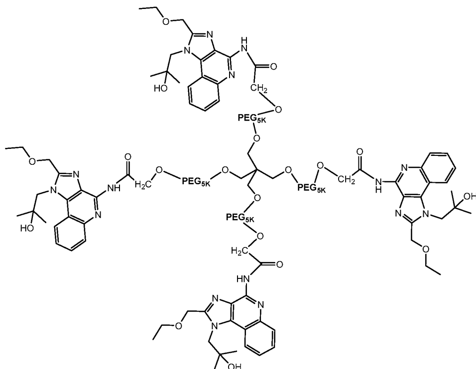
Compound 1
