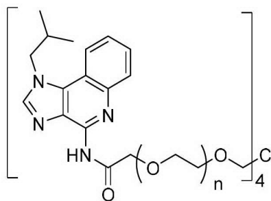
Compound 15
