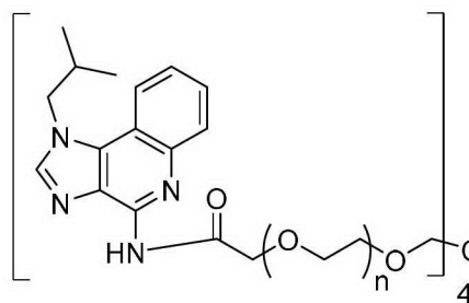
Compound 14
