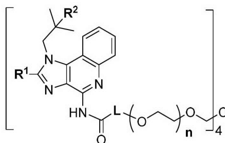
(Formula III)
