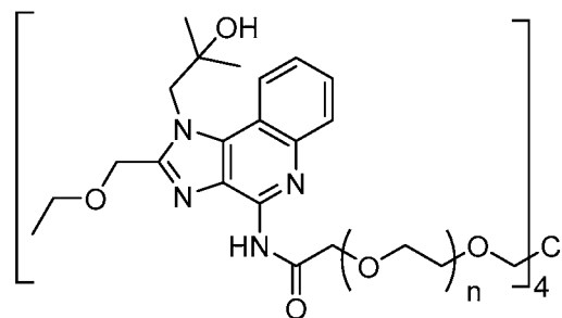
Compound 5
