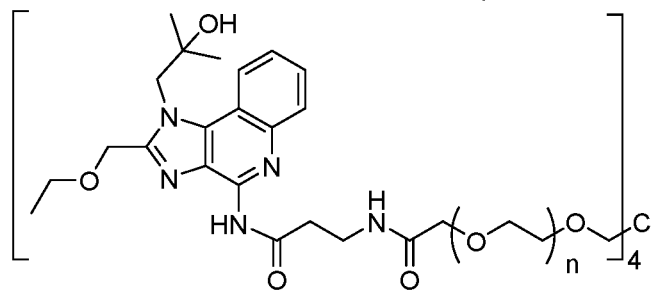
Compound 1
