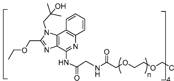
Compound 6
