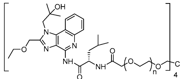
Compound 9
