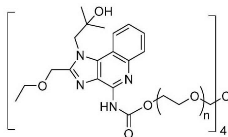
Compound 12
