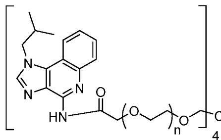
Compound 14
