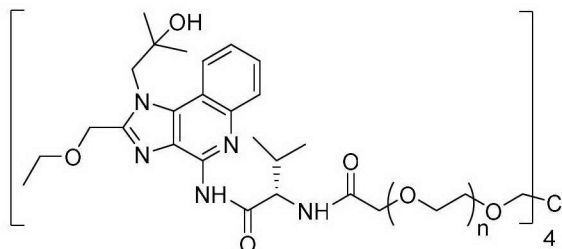
Compound 8
