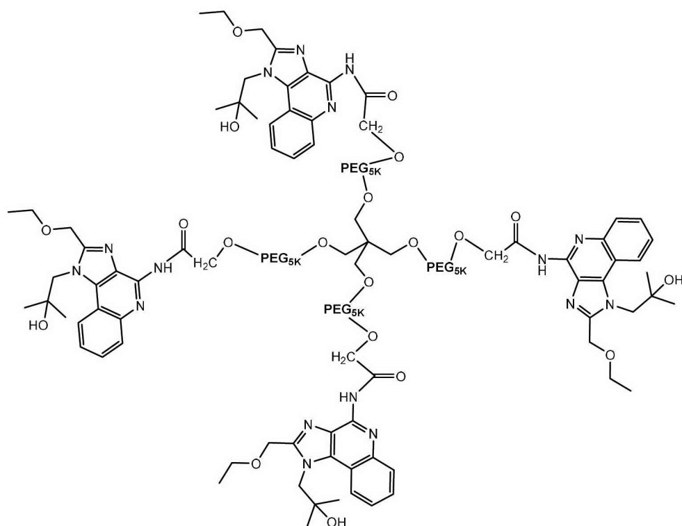
Compound 1
