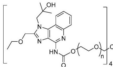
Compound 12
