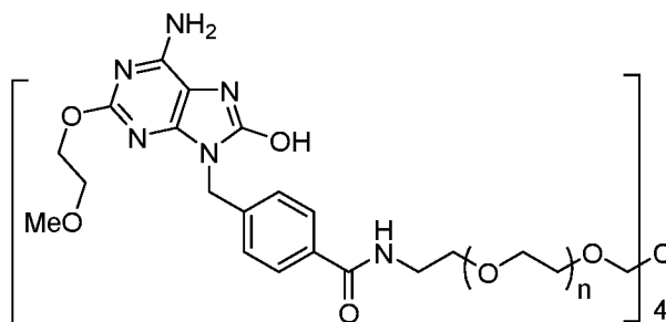
Compound 16
