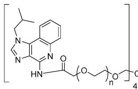
Compound 14
