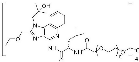
Compound 9
