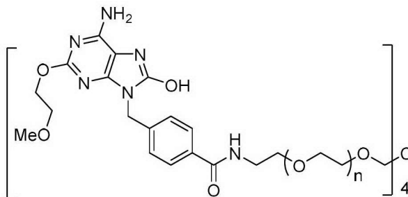
Compound 16
