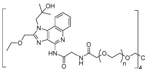
Compound 6
