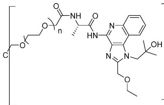
Compound 7
