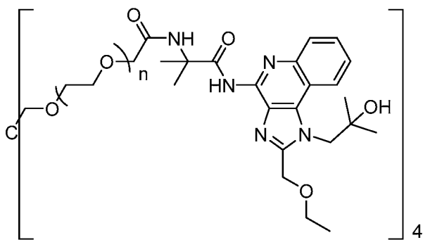
Compound 10
