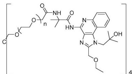
Compound 10
