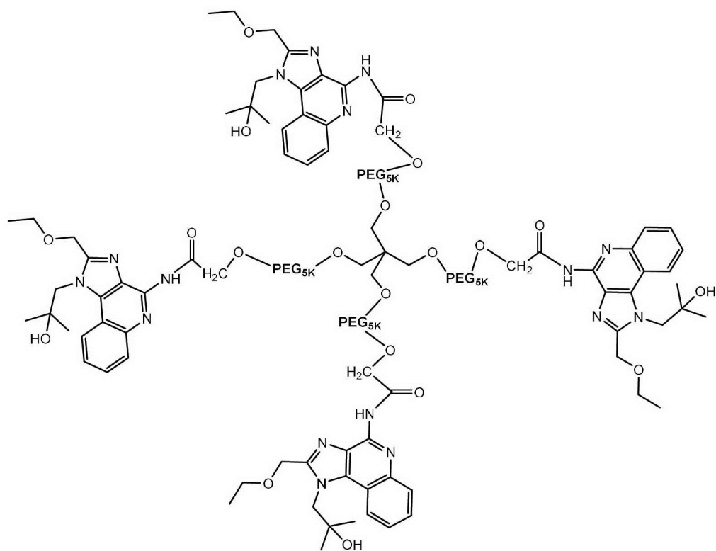
Compound 1
