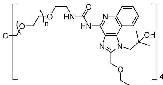
Compound 13
