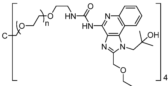
Compound 13
