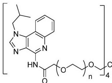
Compound 15
