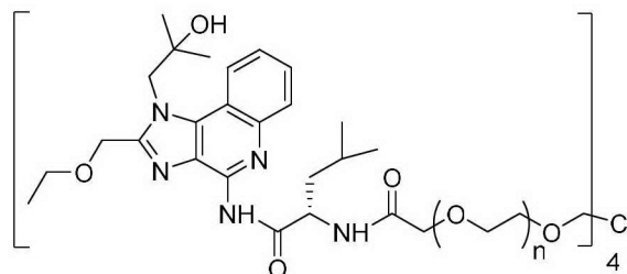
Compound 9
