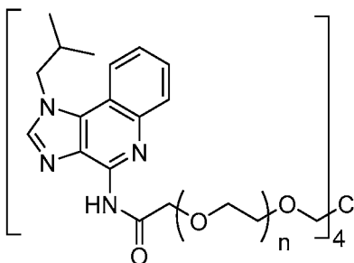
Compound 15
