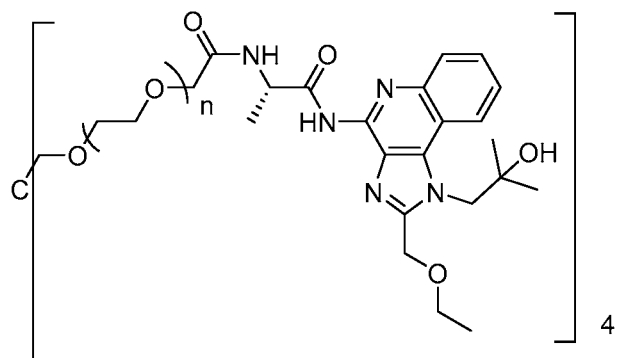
Compound 7
