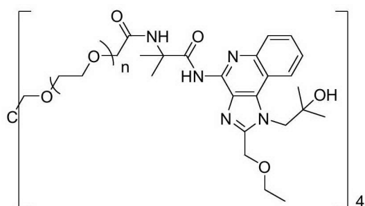
Compound 10
