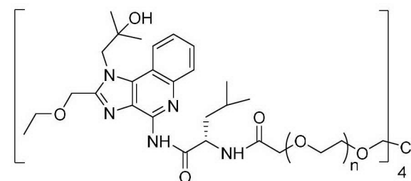
Compound 9
