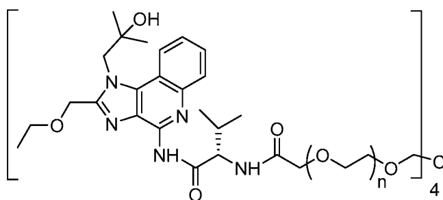
Compound 8
