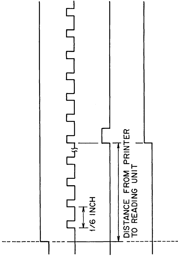
CONVEYANCE PULSE SIGNAL AT EVERY 1/6 INCH
