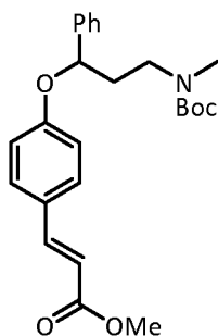
(E)-Methyl 3-[4-[3-[ tert -butoxycarbonyl(methyl)amino]-1-phenylpropoxy]phenyl]acrylate
